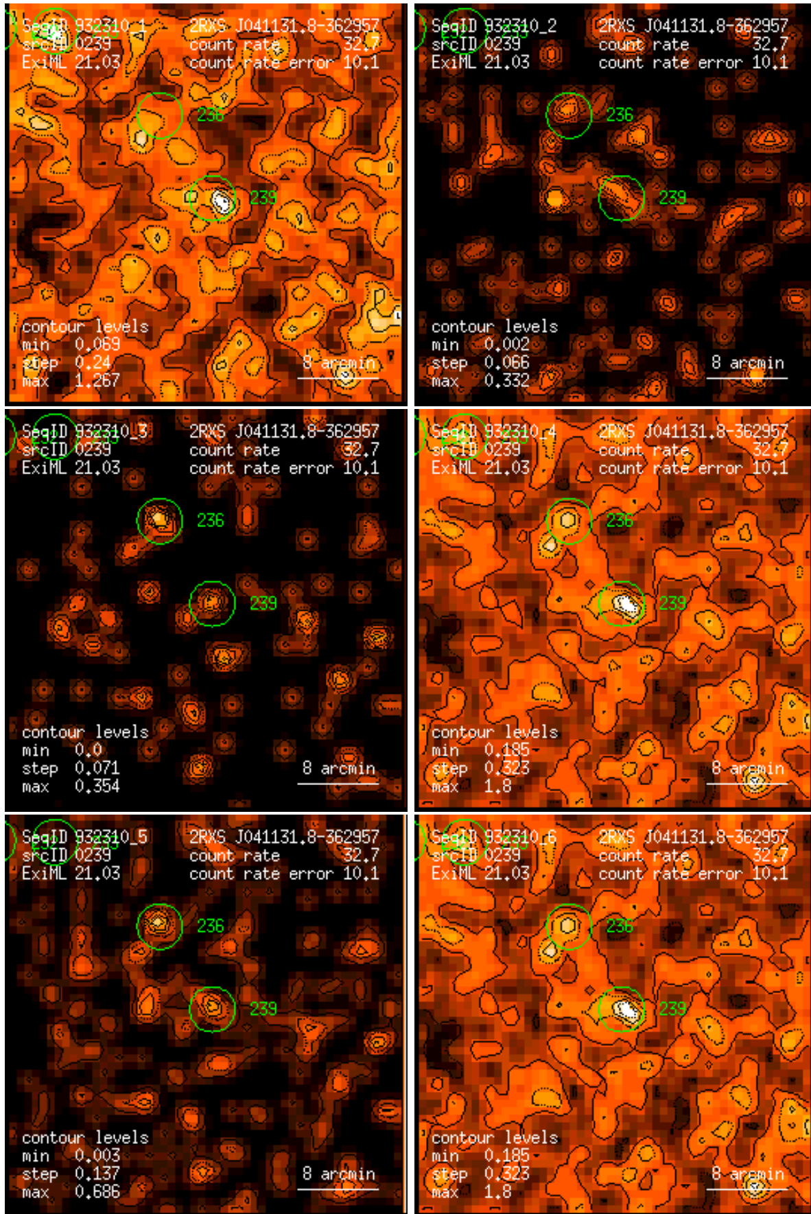
Figure 239: RASS 932310: detection 0239: band rate images, Gaussian filter: (1) PSPC channels 11 – 41, (2) 52 – 90, (3) 91 – 201, (4) 11 – 235, (5) 52 – 201, (6) 11 – 201. Broad band rates in counts/ks. Band rate contour levels in counts/ks/arcmin 2 .
