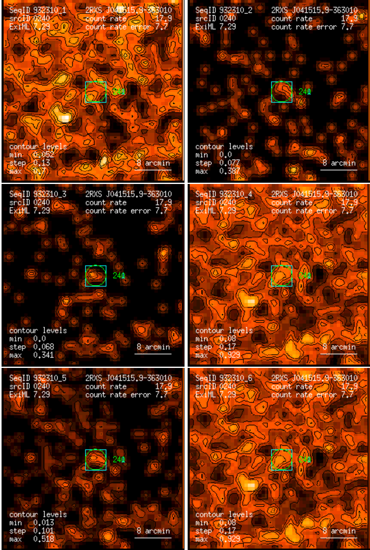
Figure 240: RASS 932310: detection 0240: band rate images, Gaussian filter: (1) PSPC channels 11 – 41, (2) 52 – 90, (3) 91 – 201, (4) 11 – 235, (5) 52 – 201, (6) 11 – 201. Broad band rates in counts/ks. Band rate contour levels in counts/ks/arcmin 2 .
