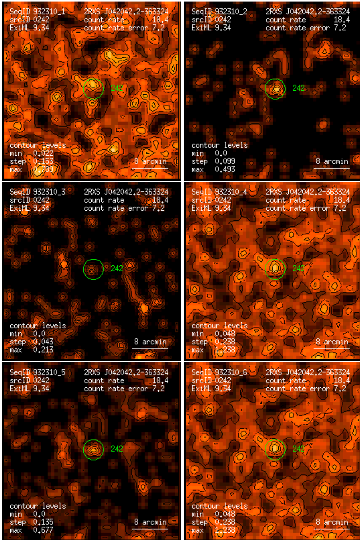
Figure 242: RASS 932310: detection 0242: band rate images, Gaussian filter: (1) PSPC channels 11 – 41, (2) 52 – 90, (3) 91 – 201, (4) 11 – 235, (5) 52 – 201, (6) 11 – 201. Broad band rates in counts/ks. Band rate contour levels in counts/ks/arcmin 2 .
