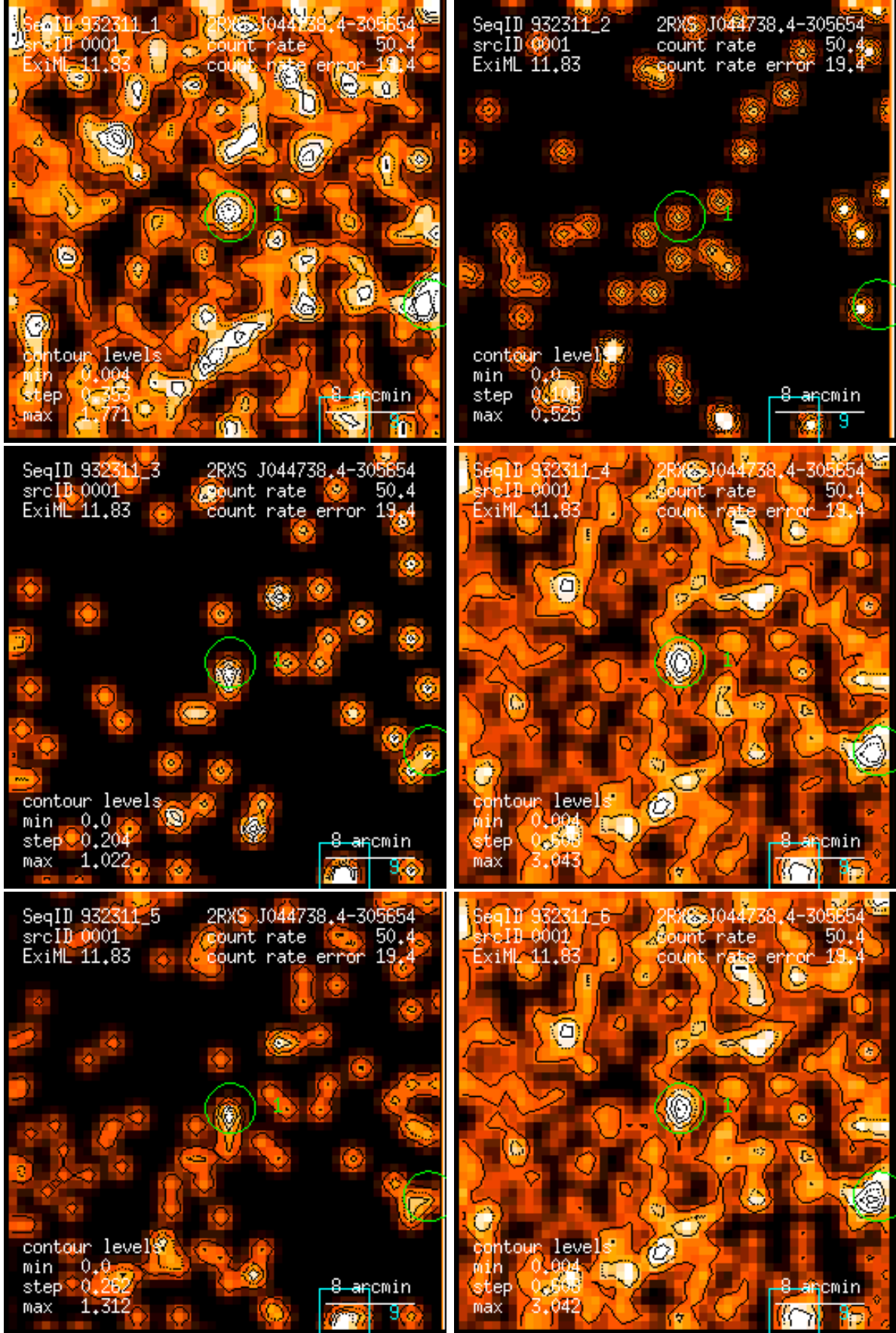
Figure 1: RASS 932311: detection 0001: band rate images, Gaussian filter: (1) PSPC channels 11 – 41, (2) 52 – 90, (3) 91 – 201, (4) 11 – 235, (5) 52 – 201, (6) 11 – 201. Broad band rates in counts/ks. Band rate contour levels in counts/ks/arcmin 2 .
