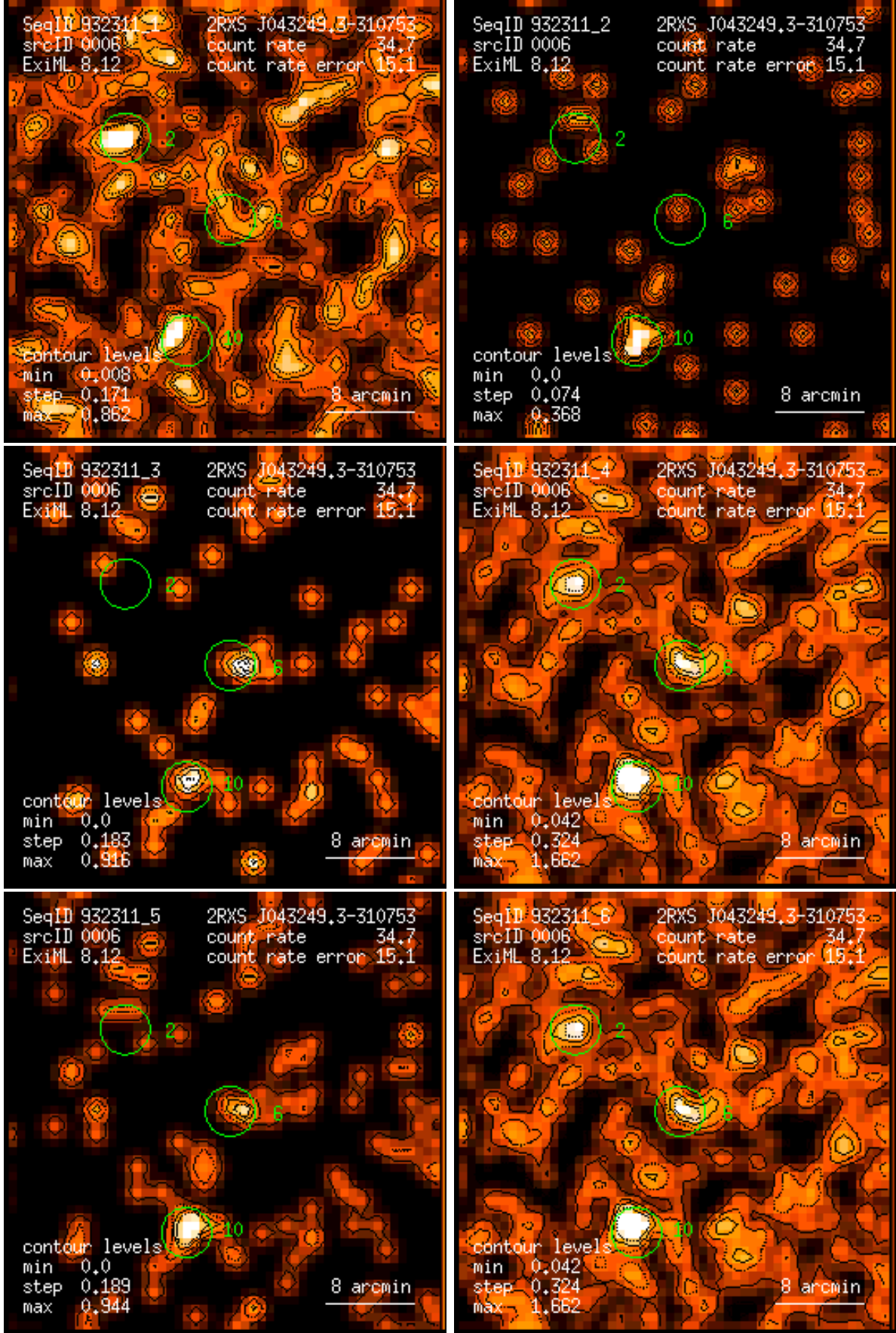
Figure 6: RASS 932311: detection 0006: band rate images, Gaussian filter: (1) PSPC channels 11 – 41, (2) 52 – 90, (3) 91 – 201, (4) 11 – 235, (5) 52 – 201, (6) 11 – 201. Broad band rates in counts/ks. Band rate contour levels in counts/ks/arcmin 2 .
