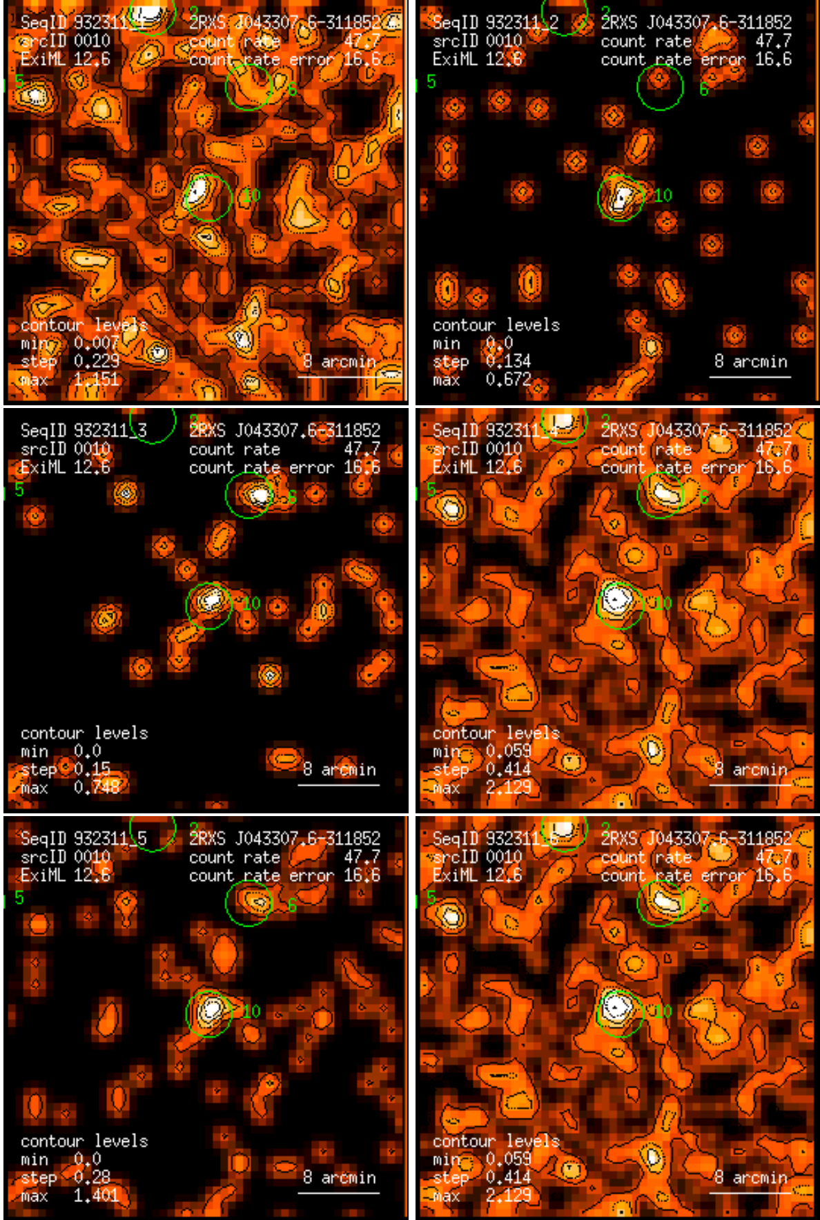
Figure 10: RASS 932311: detection 0010: band rate images, Gaussian filter: (1) PSPC channels 11 – 41, (2) 52 – 90, (3) 91 – 201, (4) 11 – 235, (5) 52 – 201, (6) 11 – 201. Broad band rates in counts/ks. Band rate contour levels in counts/ks/arcmin 2 .
