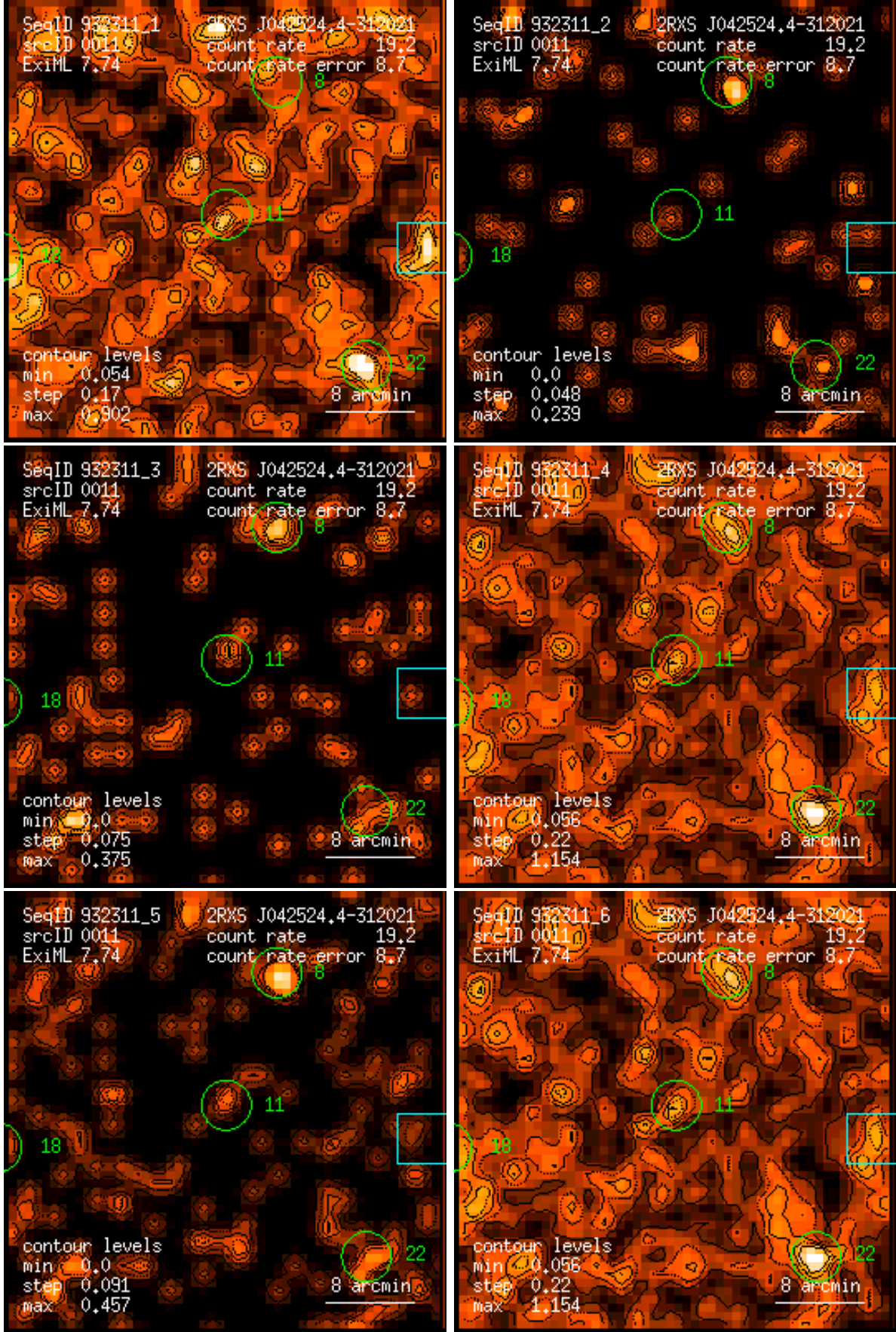
Figure 11: RASS 932311: detection 0011: band rate images, Gaussian filter: (1) PSPC channels 11 – 41, (2) 52 – 90, (3) 91 – 201, (4) 11 – 235, (5) 52 – 201, (6) 11 – 201. Broad band rates in counts/ks. Band rate contour levels in counts/ks/arcmin 2 .
