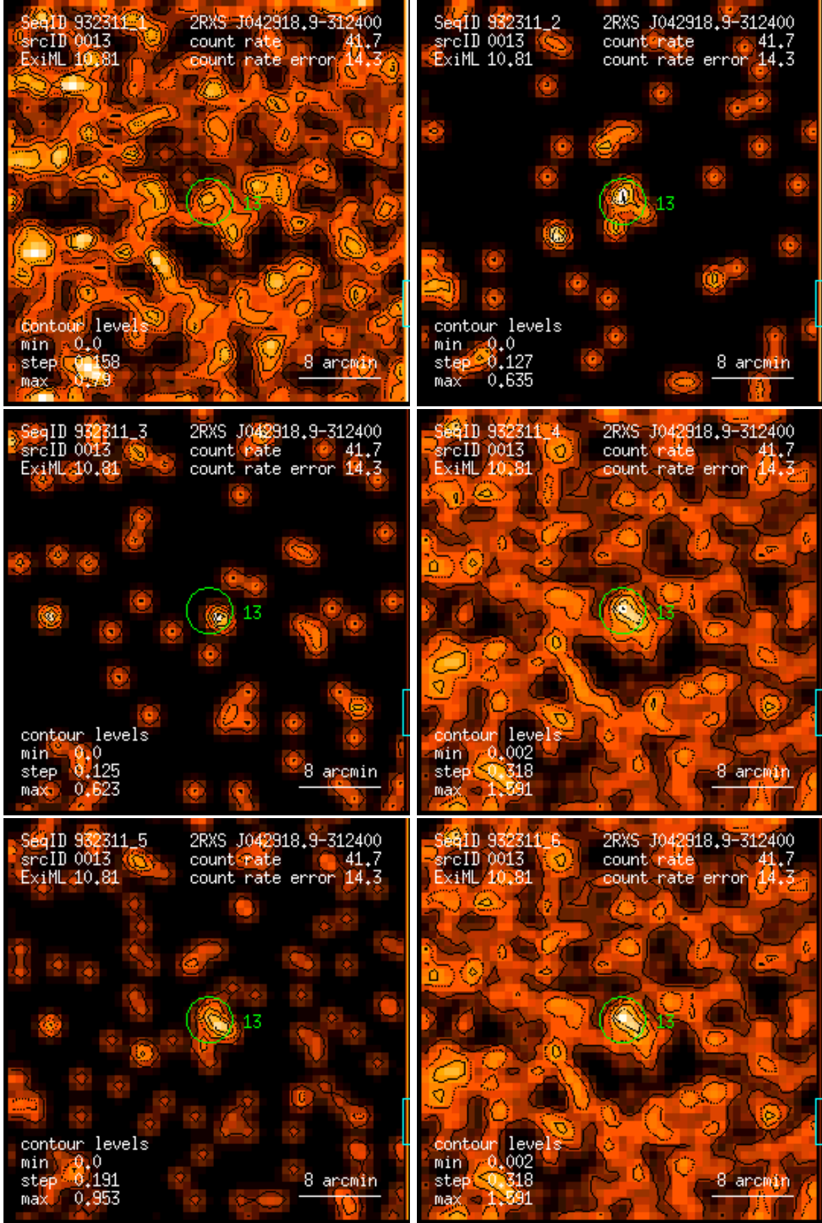
Figure 13: RASS 932311: detection 0013: band rate images, Gaussian filter: (1) PSPC channels 11 – 41, (2) 52 – 90, (3) 91 – 201, (4) 11 – 235, (5) 52 – 201, (6) 11 – 201. Broad band rates in counts/ks. Band rate contour levels in counts/ks/arcmin 2 .
