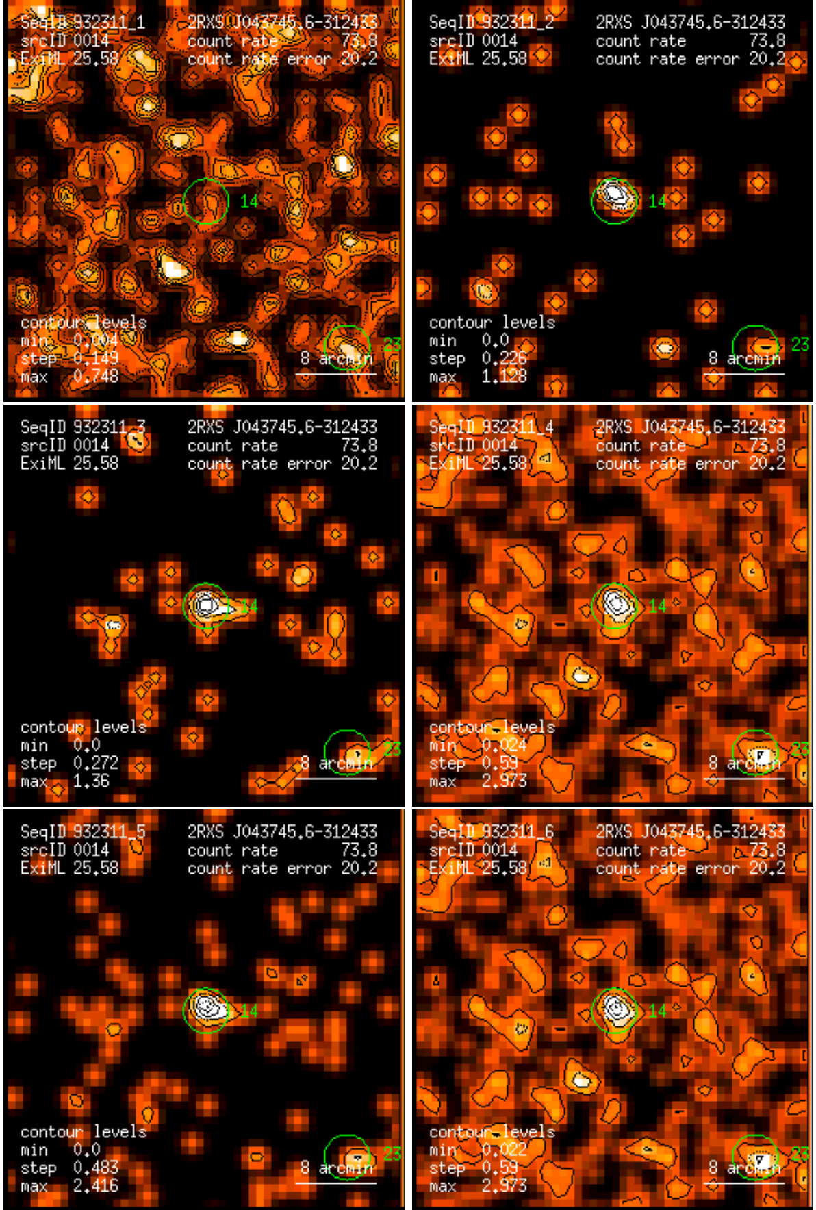
Figure 14: RASS 932311: detection 0014: band rate images, Gaussian filter: (1) PSPC channels 11 – 41, (2) 52 – 90, (3) 91 – 201, (4) 11 – 235, (5) 52 – 201, (6) 11 – 201. Broad band rates in counts/ks. Band rate contour levels in counts/ks/arcmin 2 .
