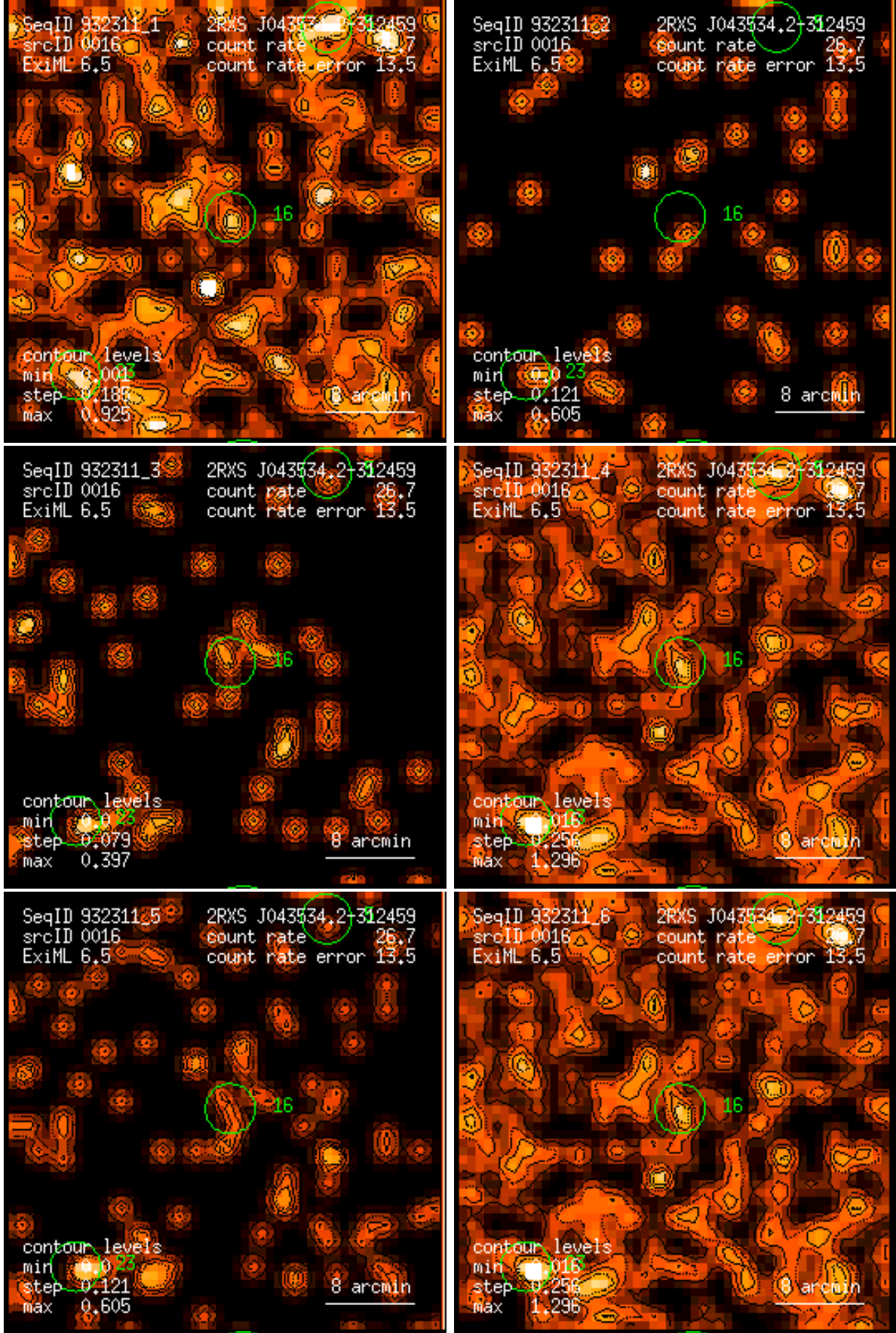
Figure 16: RASS 932311: detection 0016: band rate images, Gaussian filter: (1) PSPC channels 11 – 41, (2) 52 – 90, (3) 91 – 201, (4) 11 – 235, (5) 52 – 201, (6) 11 – 201. Broad band rates in counts/ks. Band rate contour levels in counts/ks/arcmin 2 .
