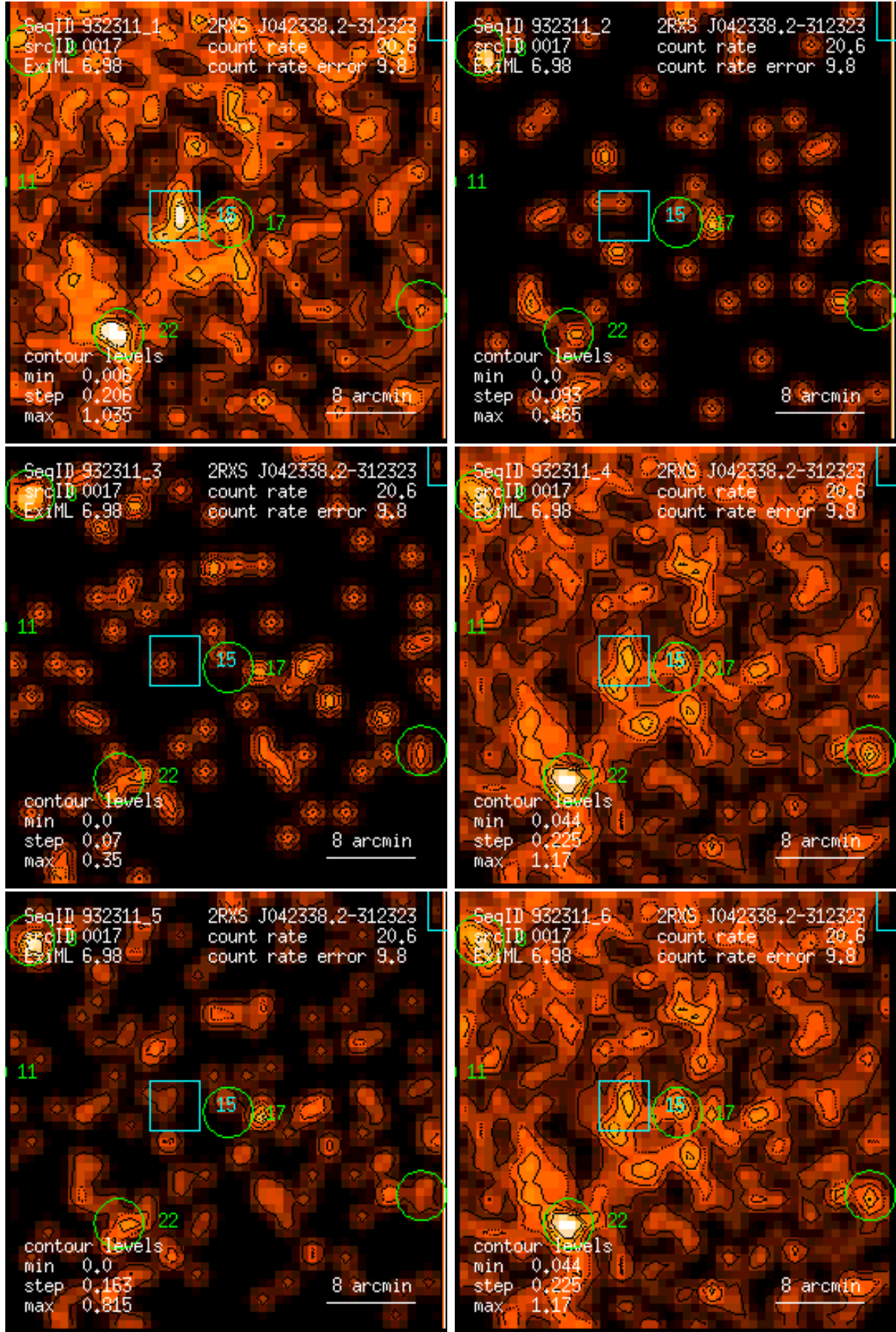
Figure 17: RASS 932311: detection 0017: band rate images, Gaussian filter: (1) PSPC channels 11 – 41, (2) 52 – 90, (3) 91 – 201, (4) 11 – 235, (5) 52 – 201, (6) 11 – 201. Broad band rates in counts/ks. Band rate contour levels in counts/ks/arcmin 2 .
