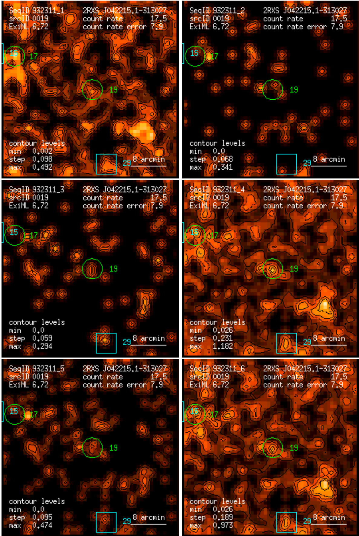
Figure 19: RASS 932311: detection 0019: band rate images, Gaussian filter: (1) PSPC channels 11 – 41, (2) 52 – 90, (3) 91 – 201, (4) 11 – 235, (5) 52 – 201, (6) 11 – 201. Broad band rates in counts/ks. Band rate contour levels in counts/ks/arcmin 2 .
