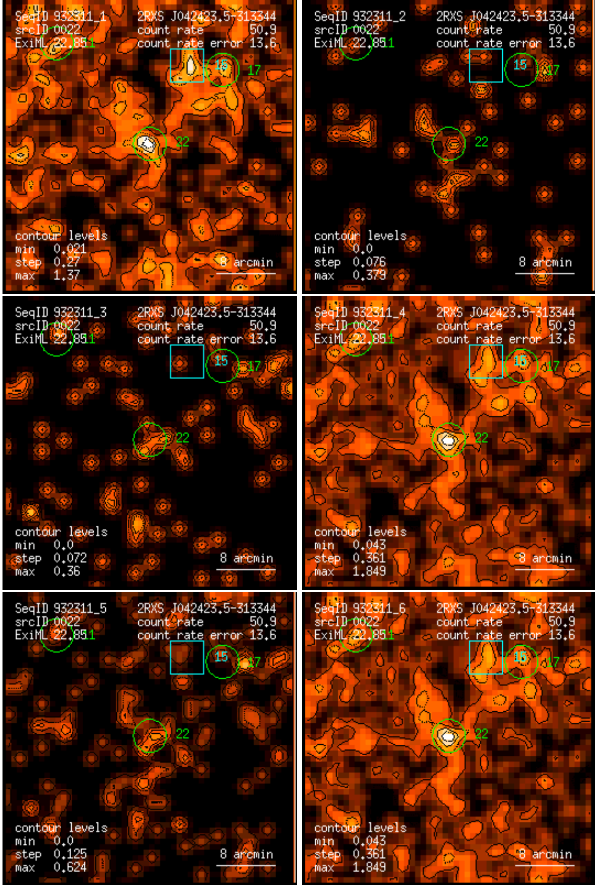
Figure 22: RASS 932311: detection 0022: band rate images, Gaussian filter: (1) PSPC channels 11 – 41, (2) 52 – 90, (3) 91 – 201, (4) 11 – 235, (5) 52 – 201, (6) 11 – 201. Broad band rates in counts/ks. Band rate contour levels in counts/ks/arcmin 2 .
