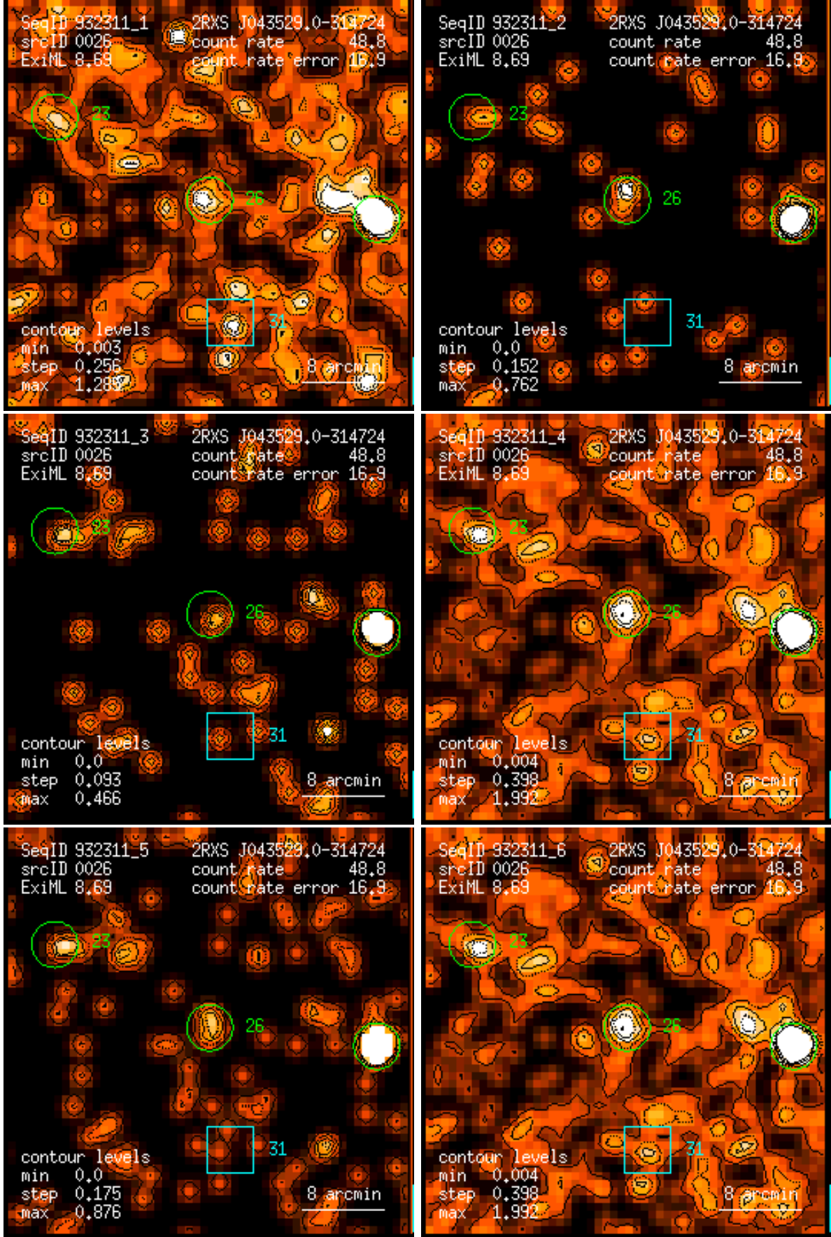
Figure 26: RASS 932311: detection 0026: band rate images, Gaussian filter: (1) PSPC channels 11 – 41, (2) 52 – 90, (3) 91 – 201, (4) 11 – 235, (5) 52 – 201, (6) 11 – 201. Broad band rates in counts/ks. Band rate contour levels in counts/ks/arcmin 2 .
