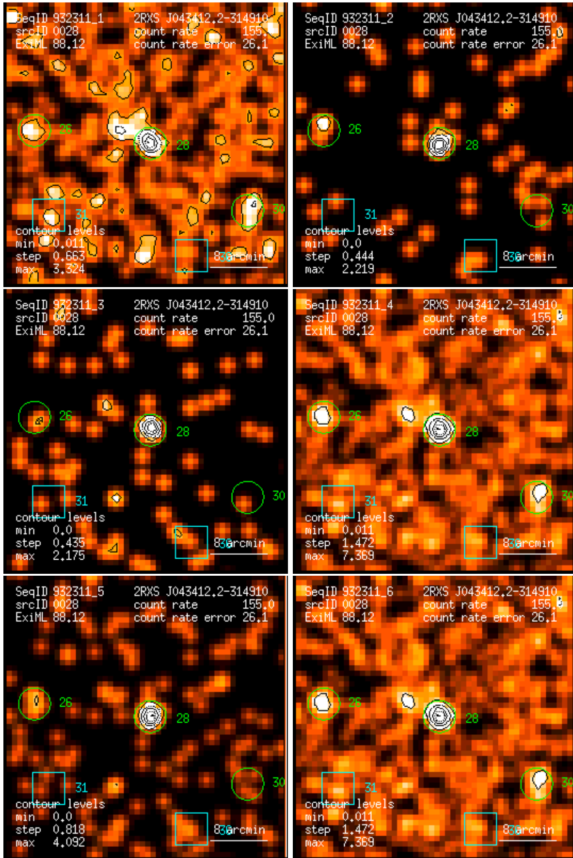
Figure 28: RASS 932311: detection 0028: band rate images, Gaussian filter: (1) PSPC channels 11 – 41, (2) 52 – 90, (3) 91 – 201, (4) 11 – 235, (5) 52 – 201, (6) 11 – 201. Broad band rates in counts/ks. Band rate contour levels in counts/ks/arcmin 2 .
