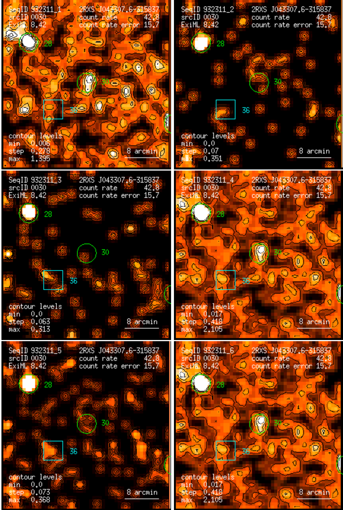
Figure 30: RASS 932311: detection 0030: band rate images, Gaussian filter: (1) PSPC channels 11 – 41, (2) 52 – 90, (3) 91 – 201, (4) 11 – 235, (5) 52 – 201, (6) 11 – 201. Broad band rates in counts/ks. Band rate contour levels in counts/ks/arcmin 2 .
