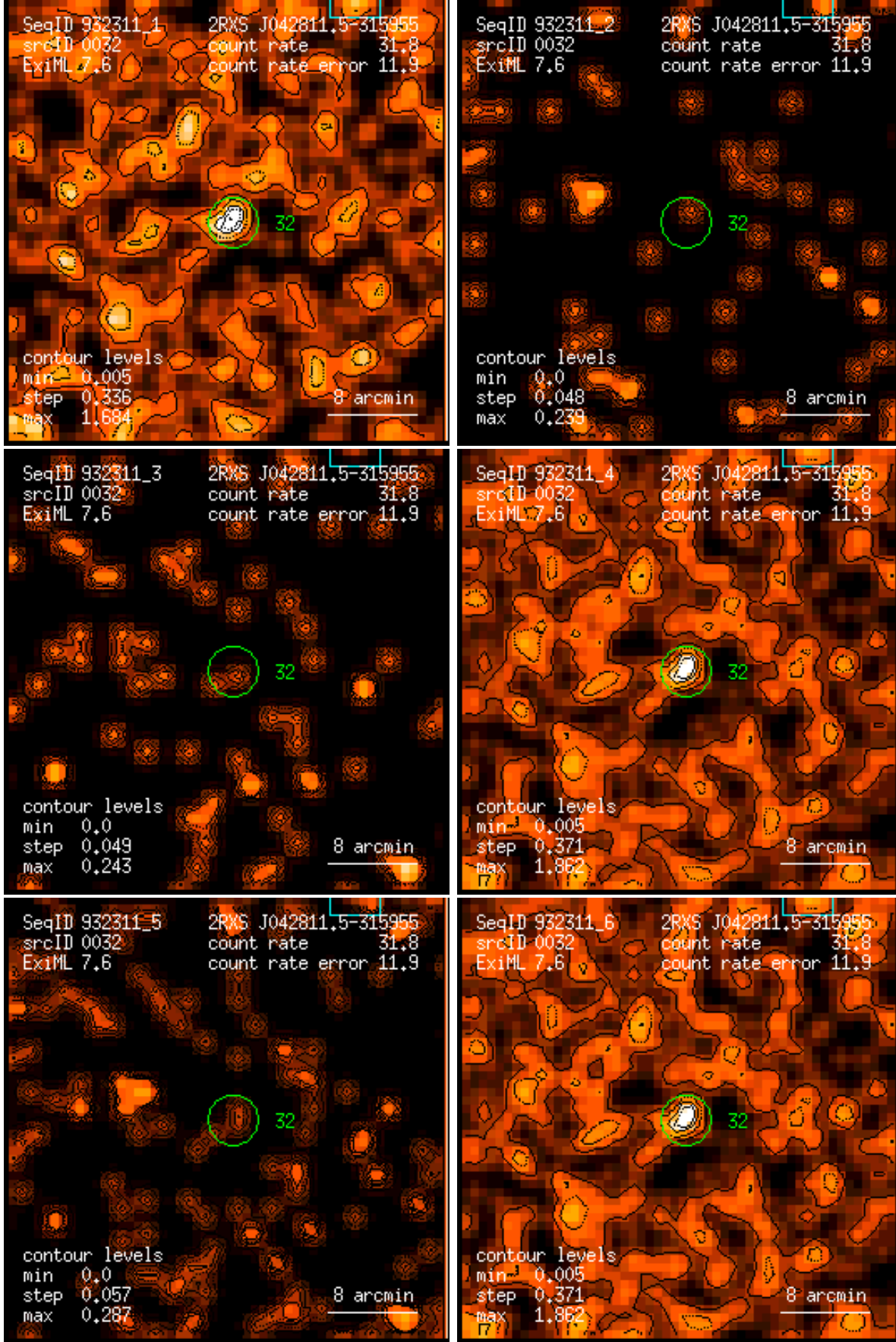
Figure 32: RASS 932311: detection 0032: band rate images, Gaussian filter: (1) PSPC channels 11 – 41, (2) 52 – 90, (3) 91 – 201, (4) 11 – 235, (5) 52 – 201, (6) 11 – 201. Broad band rates in counts/ks. Band rate contour levels in counts/ks/arcmin 2 .
