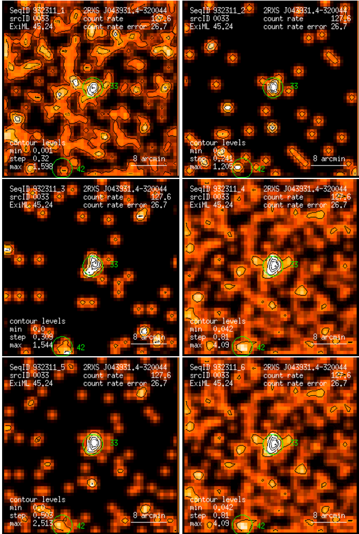
Figure 33: RASS 932311: detection 0033: band rate images, Gaussian filter: (1) PSPC channels 11 – 41, (2) 52 – 90, (3) 91 – 201, (4) 11 – 235, (5) 52 – 201, (6) 11 – 201. Broad band rates in counts/ks. Band rate contour levels in counts/ks/arcmin 2 .
