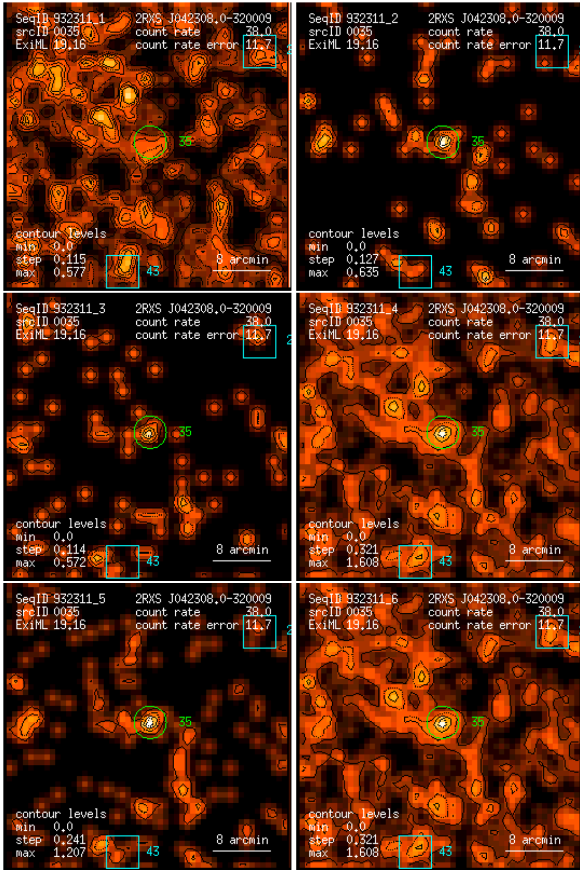
Figure 35: RASS 932311: detection 0035: band rate images, Gaussian filter: (1) PSPC channels 11 – 41, (2) 52 – 90, (3) 91 – 201, (4) 11 – 235, (5) 52 – 201, (6) 11 – 201. Broad band rates in counts/ks. Band rate contour levels in counts/ks/arcmin 2 .
