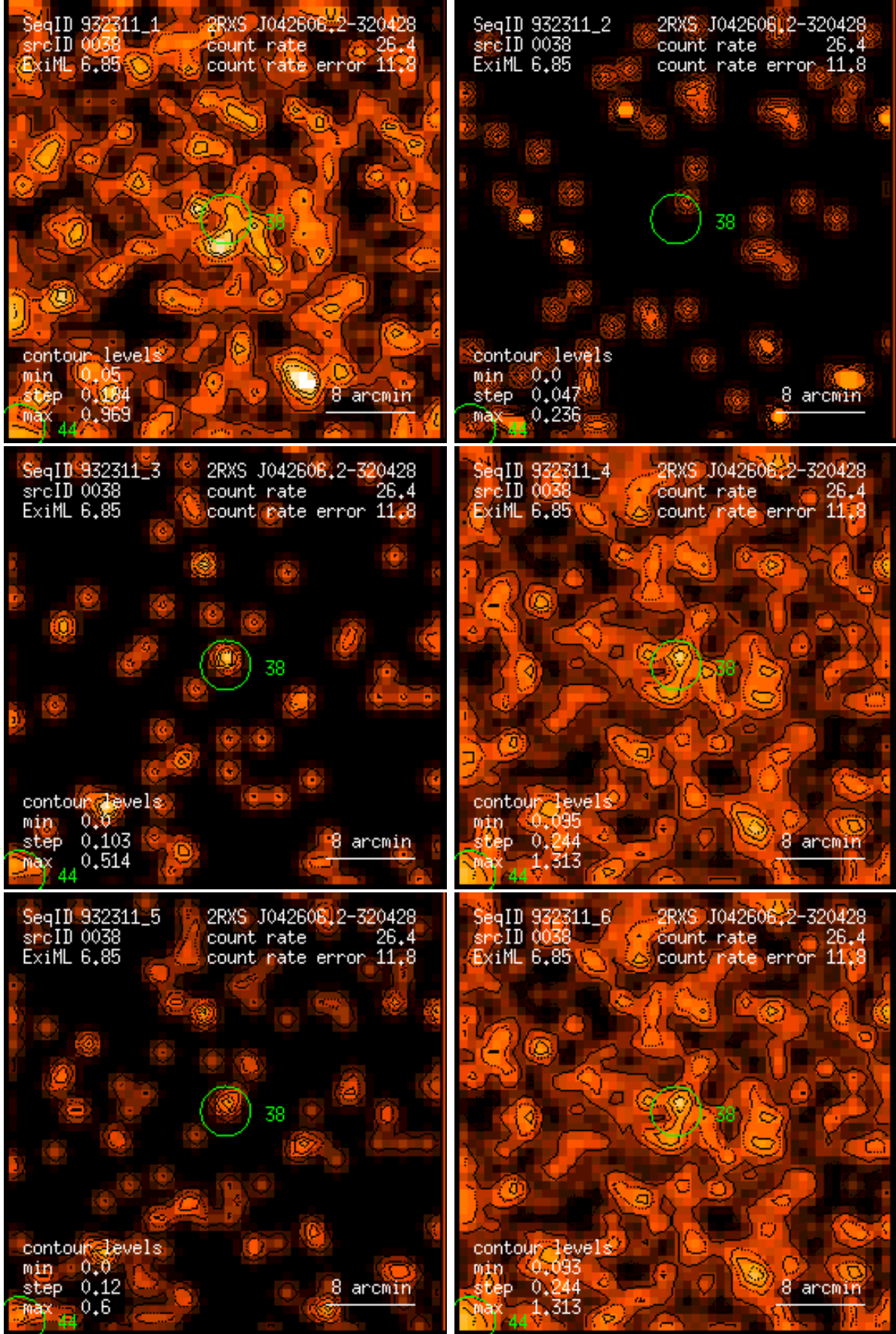
Figure 38: RASS 932311: detection 0038: band rate images, Gaussian filter: (1) PSPC channels 11 – 41, (2) 52 – 90, (3) 91 – 201, (4) 11 – 235, (5) 52 – 201, (6) 11 – 201. Broad band rates in counts/ks. Band rate contour levels in counts/ks/arcmin 2 .
