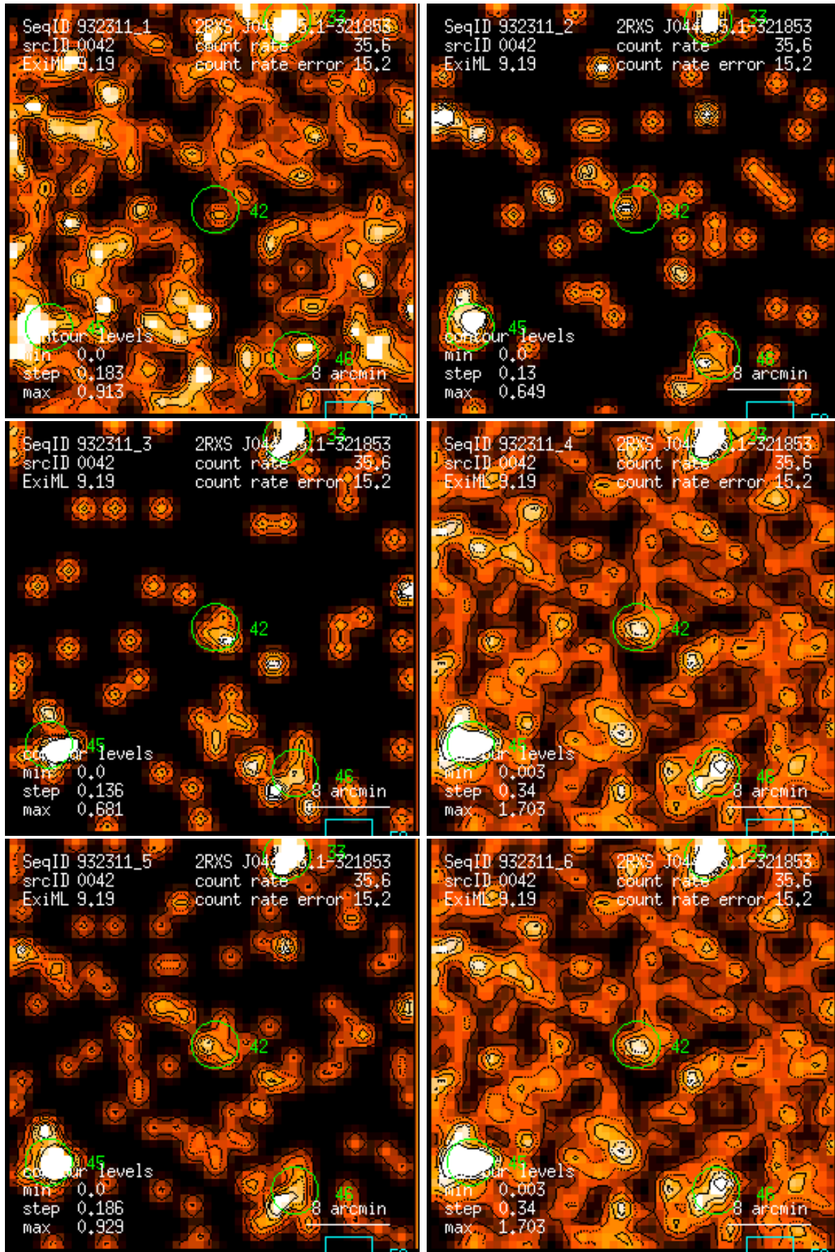
Figure 42: RASS 932311: detection 0042: band rate images, Gaussian filter: (1) PSPC channels 11 – 41, (2) 52 – 90, (3) 91 – 201, (4) 11 – 235, (5) 52 – 201, (6) 11 – 201. Broad band rates in counts/ks. Band rate contour levels in counts/ks/arcmin 2 .
