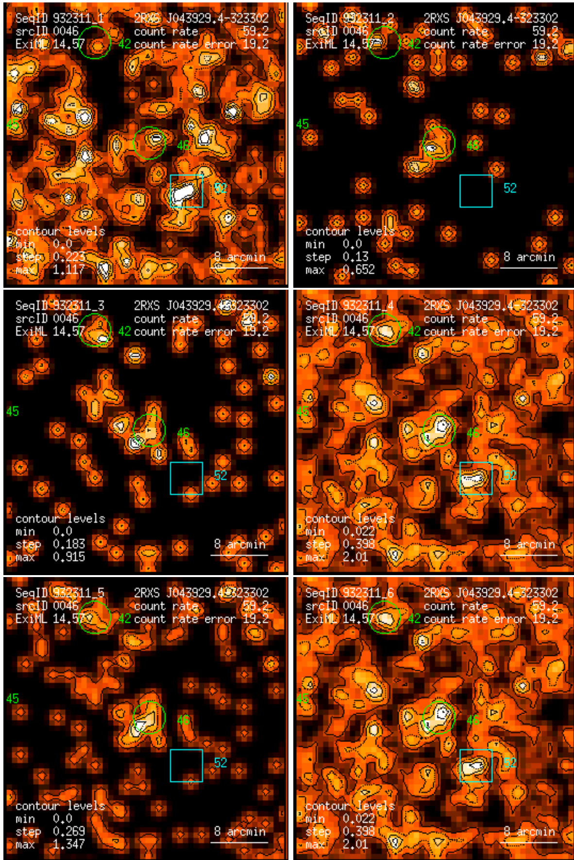
Figure 46: RASS 932311: detection 0046: band rate images, Gaussian filter: (1) PSPC channels 11 – 41, (2) 52 – 90, (3) 91 – 201, (4) 11 – 235, (5) 52 – 201, (6) 11 – 201. Broad band rates in counts/ks. Band rate contour levels in counts/ks/arcmin 2 .
