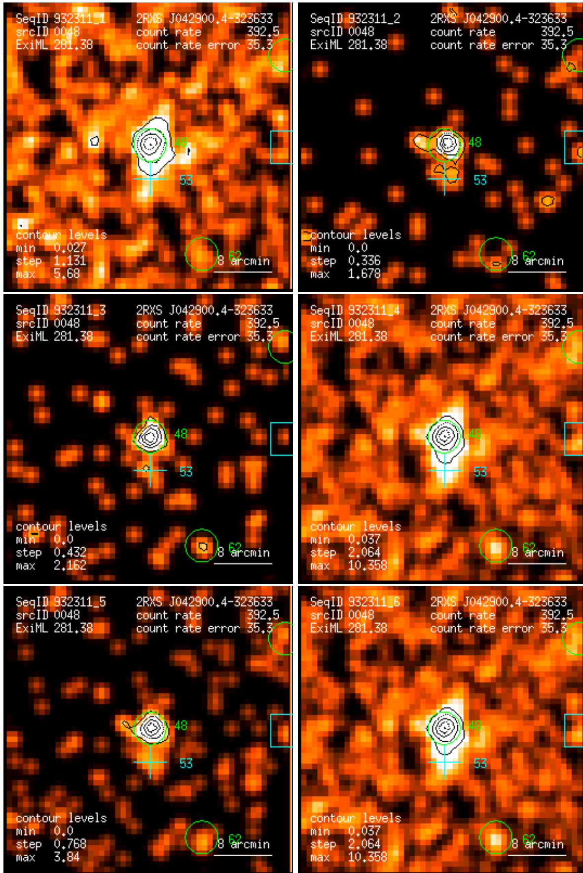
Figure 48: RASS 932311: detection 0048: band rate images, Gaussian filter: (1) PSPC channels 11 – 41, (2) 52 – 90, (3) 91 – 201, (4) 11 – 235, (5) 52 – 201, (6) 11 – 201. Broad band rates in counts/ks. Band rate contour levels in counts/ks/arcmin 2 .
