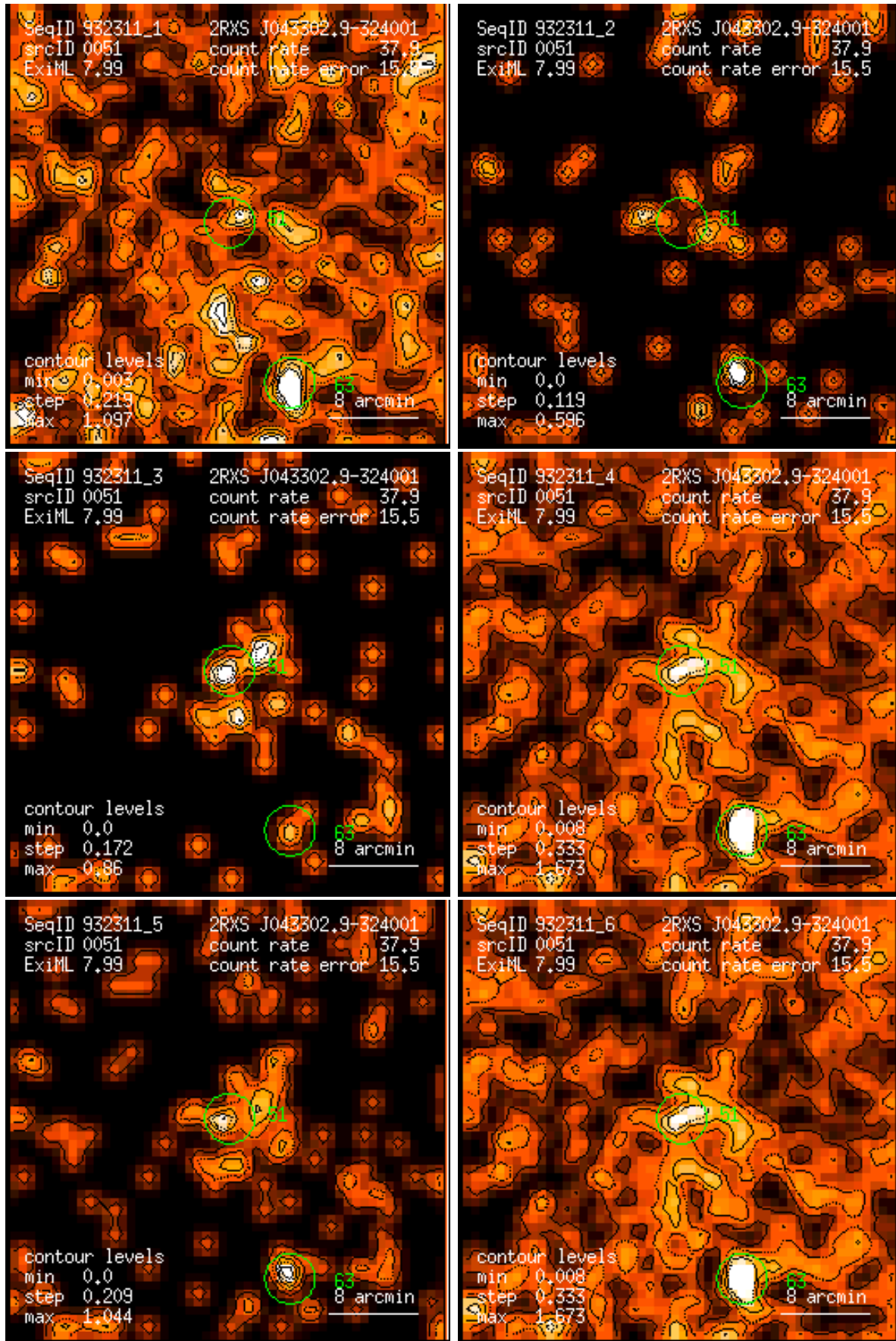
Figure 51: RASS 932311: detection 0051: band rate images, Gaussian filter: (1) PSPC channels 11 – 41, (2) 52 – 90, (3) 91 – 201, (4) 11 – 235, (5) 52 – 201, (6) 11 – 201. Broad band rates in counts/ks. Band rate contour levels in counts/ks/arcmin 2 .
