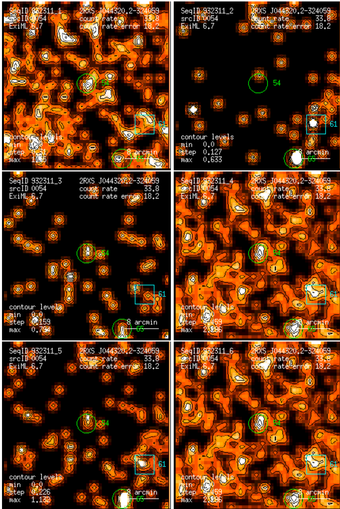
Figure 54: RASS 932311: detection 0054: band rate images, Gaussian filter: (1) PSPC channels 11 – 41, (2) 52 – 90, (3) 91 – 201, (4) 11 – 235, (5) 52 – 201, (6) 11 – 201. Broad band rates in counts/ks. Band rate contour levels in counts/ks/arcmin 2 .
