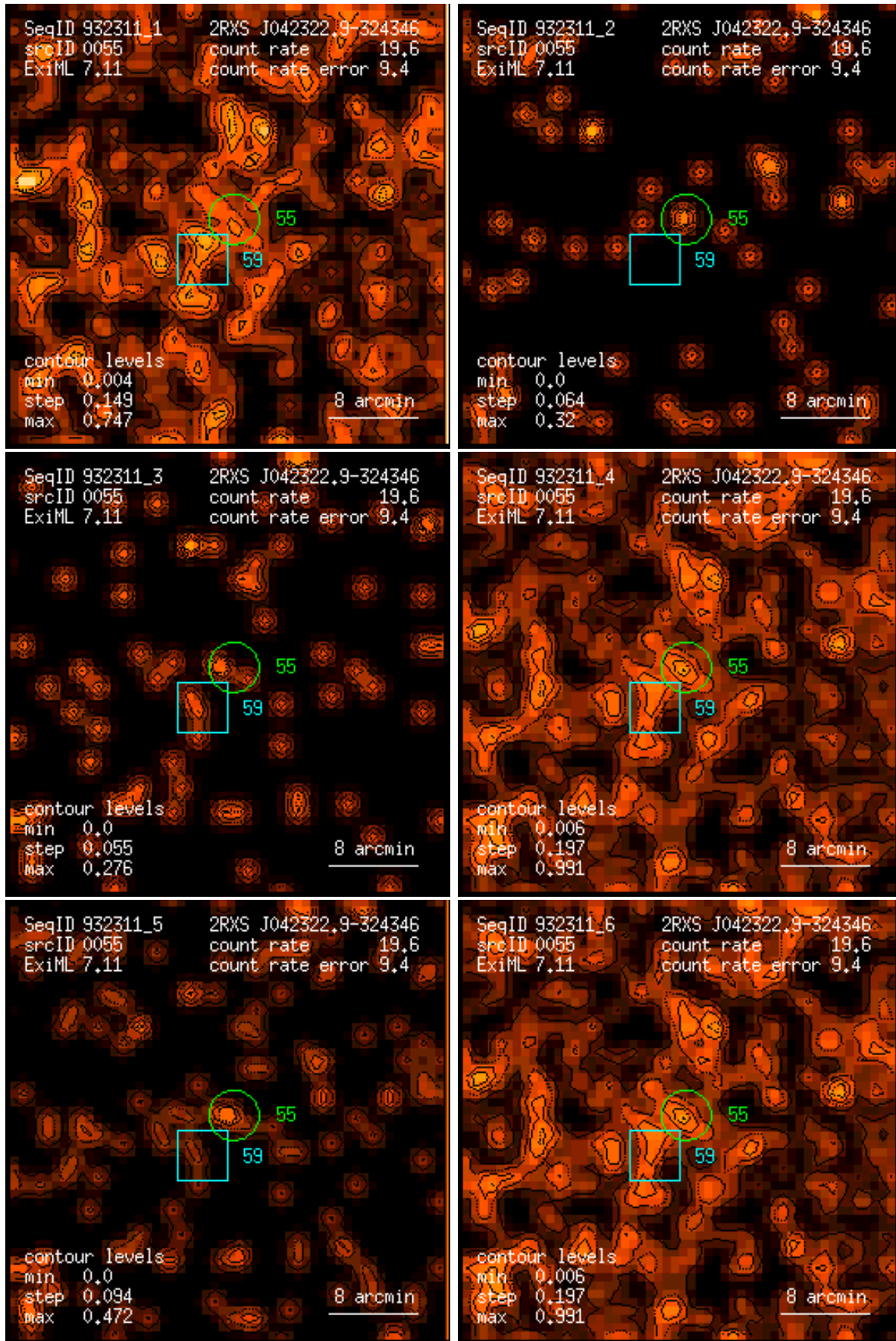
Figure 55: RASS 932311: detection 0055: band rate images, Gaussian filter: (1) PSPC channels 11 – 41, (2) 52 – 90, (3) 91 – 201, (4) 11 – 235, (5) 52 – 201, (6) 11 – 201. Broad band rates in counts/ks. Band rate contour levels in counts/ks/arcmin 2 .
