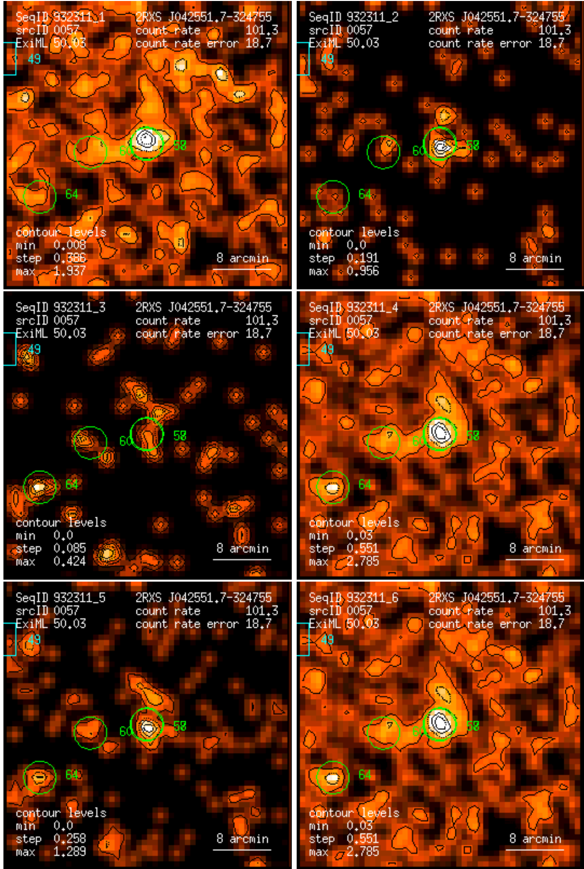
Figure 57: RASS 932311: detection 0057: band rate images, Gaussian filter: (1) PSPC channels 11 – 41, (2) 52 – 90, (3) 91 – 201, (4) 11 – 235, (5) 52 – 201, (6) 11 – 201. Broad band rates in counts/ks. Band rate contour levels in counts/ks/arcmin 2 .
