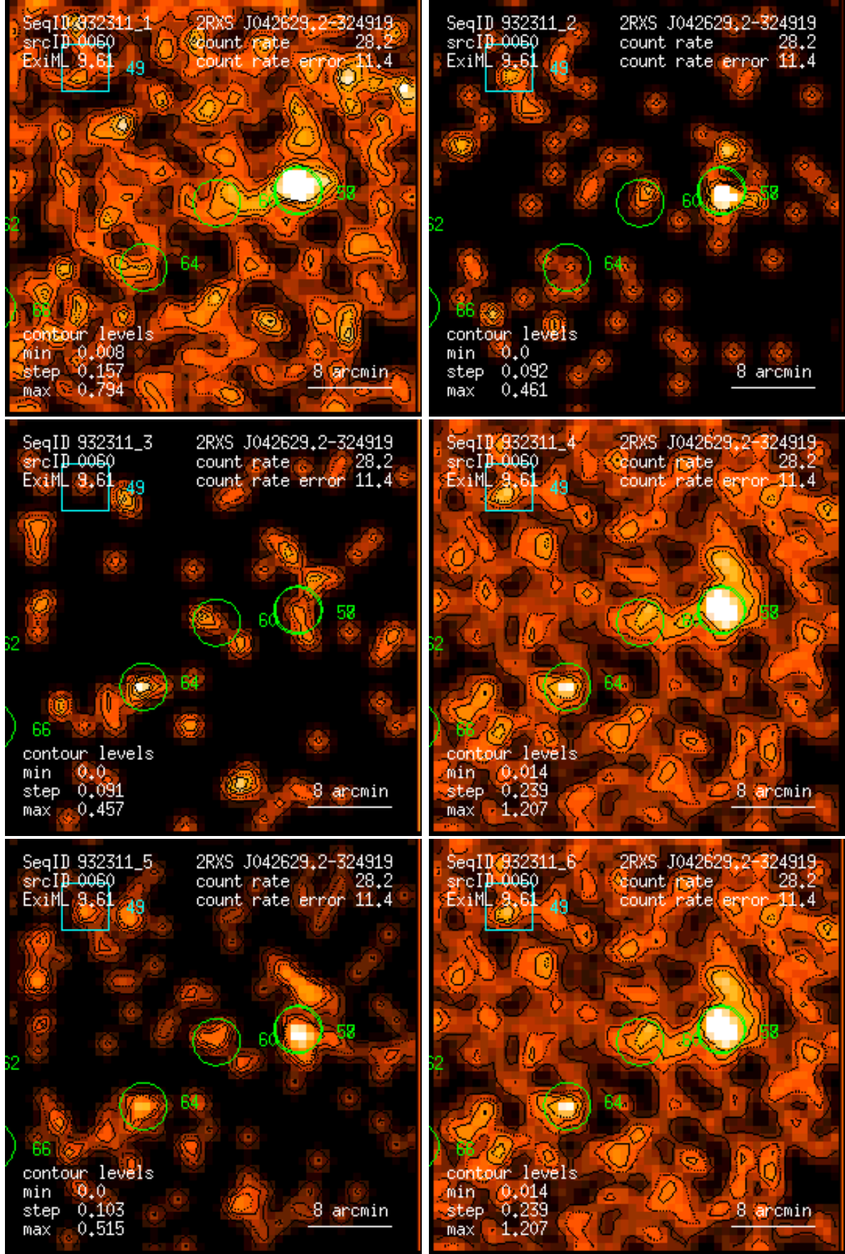
Figure 60: RASS 932311: detection 0060: band rate images, Gaussian filter: (1) PSPC channels 11 – 41, (2) 52 – 90, (3) 91 – 201, (4) 11 – 235, (5) 52 – 201, (6) 11 – 201. Broad band rates in counts/ks. Band rate contour levels in counts/ks/arcmin 2 .
