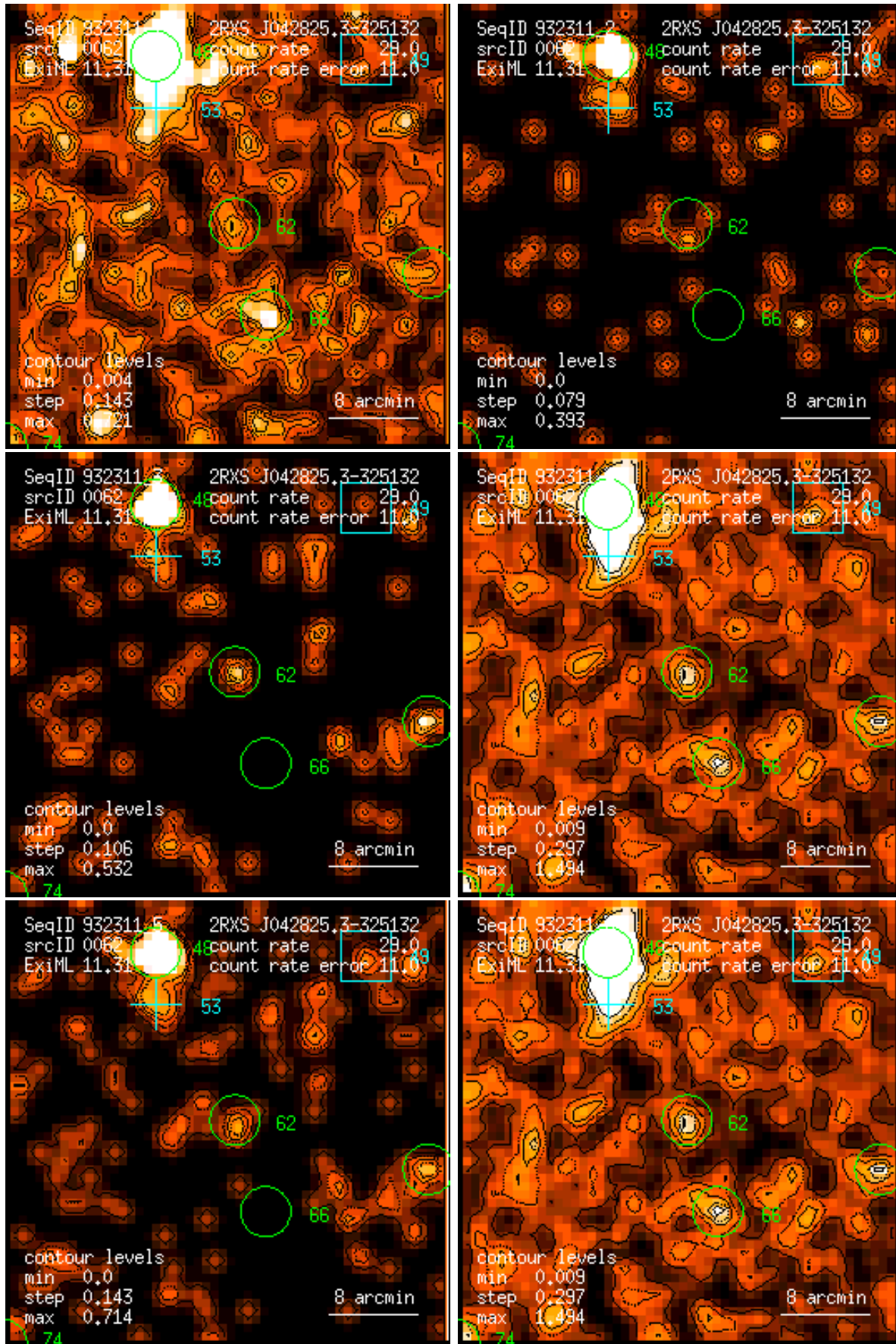
Figure 62: RASS 932311: detection 0062: band rate images, Gaussian filter: (1) PSPC channels 11 – 41, (2) 52 – 90, (3) 91 – 201, (4) 11 – 235, (5) 52 – 201, (6) 11 – 201. Broad band rates in counts/ks. Band rate contour levels in counts/ks/arcmin 2 .
