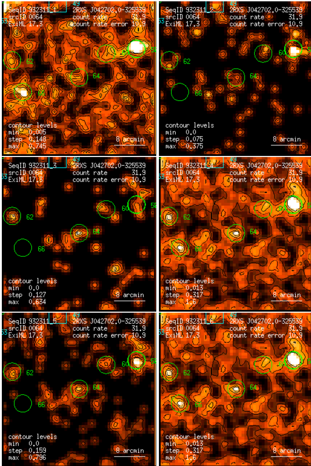
Figure 64: RASS 932311: detection 0064: band rate images, Gaussian filter: (1) PSPC channels 11 – 41, (2) 52 – 90, (3) 91 – 201, (4) 11 – 235, (5) 52 – 201, (6) 11 – 201. Broad band rates in counts/ks. Band rate contour levels in counts/ks/arcmin 2 .
