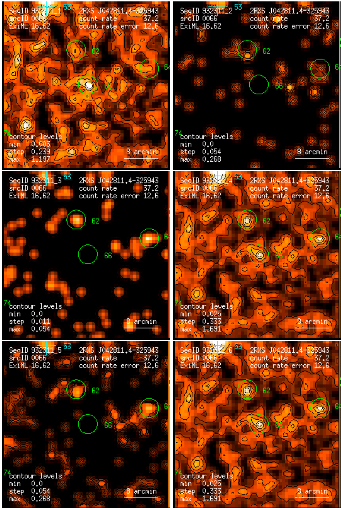
Figure 66: RASS 932311: detection 0066: band rate images, Gaussian filter: (1) PSPC channels 11 – 41, (2) 52 – 90, (3) 91 – 201, (4) 11 – 235, (5) 52 – 201, (6) 11 – 201. Broad band rates in counts/ks. Band rate contour levels in counts/ks/arcmin 2 .
