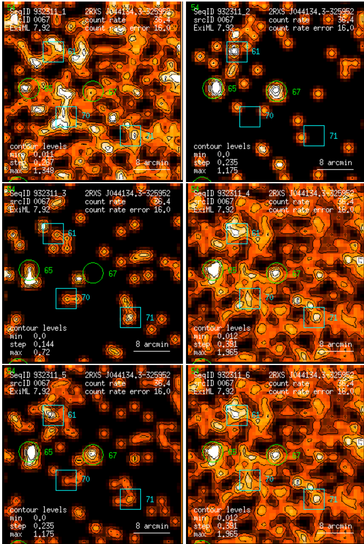
Figure 67: RASS 932311: detection 0067: band rate images, Gaussian filter: (1) PSPC channels 11 – 41, (2) 52 – 90, (3) 91 – 201, (4) 11 – 235, (5) 52 – 201, (6) 11 – 201. Broad band rates in counts/ks. Band rate contour levels in counts/ks/arcmin 2 .
