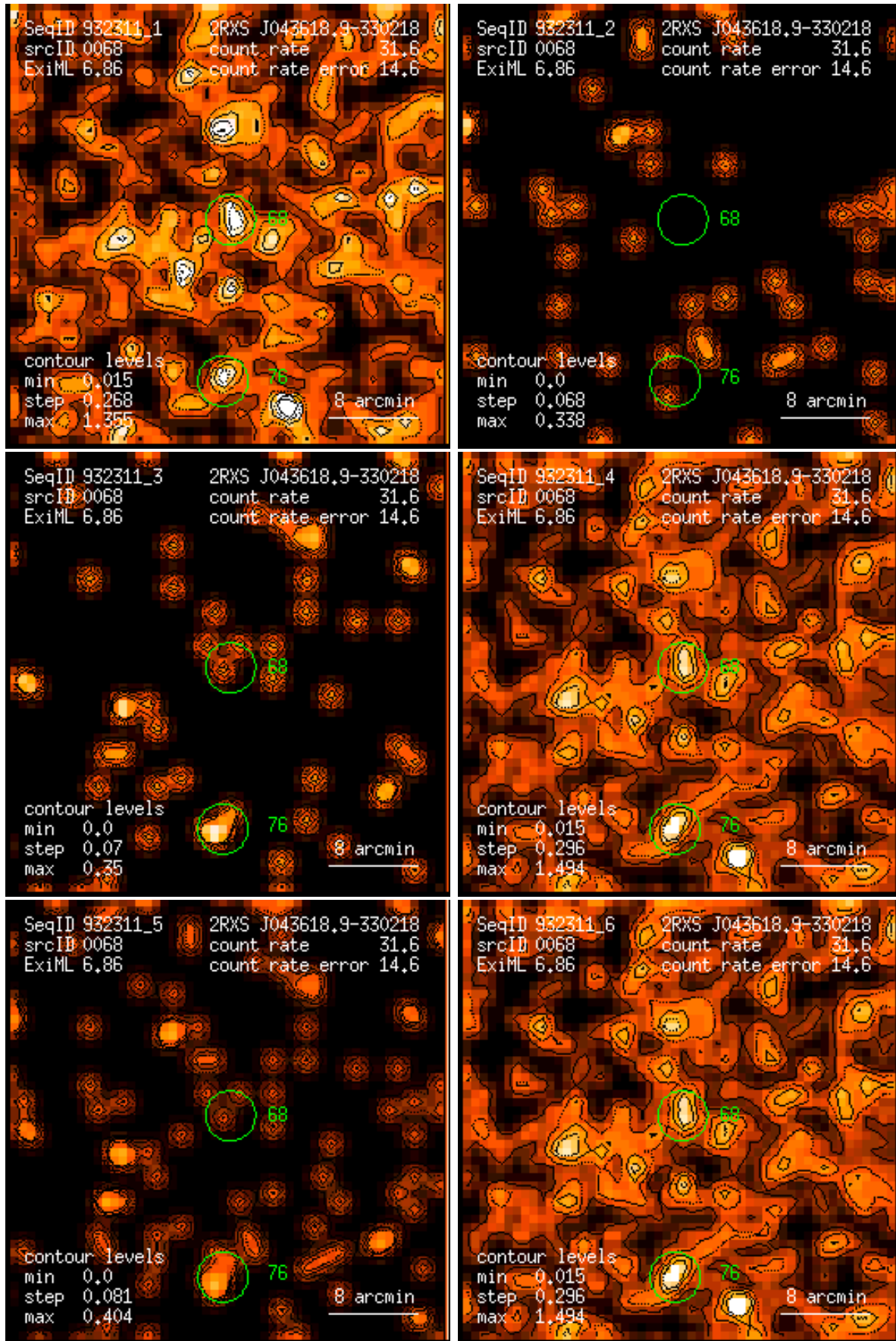
Figure 68: RASS 932311: detection 0068: band rate images, Gaussian filter: (1) PSPC channels 11 – 41, (2) 52 – 90, (3) 91 – 201, (4) 11 – 235, (5) 52 – 201, (6) 11 – 201. Broad band rates in counts/ks. Band rate contour levels in counts/ks/arcmin 2 .
