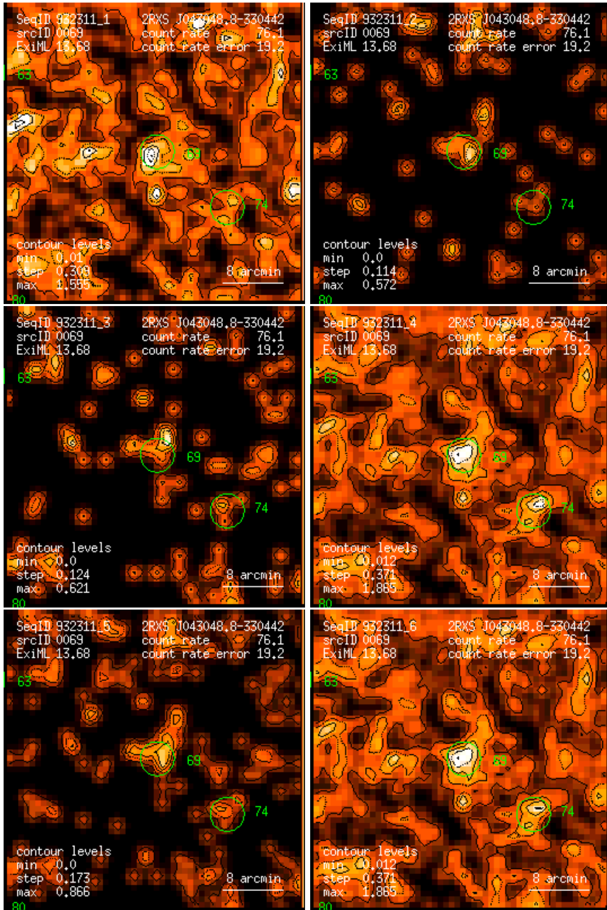
Figure 69: RASS 932311: detection 0069: band rate images, Gaussian filter: (1) PSPC channels 11 – 41, (2) 52 – 90, (3) 91 – 201, (4) 11 – 235, (5) 52 – 201, (6) 11 – 201. Broad band rates in counts/ks. Band rate contour levels in counts/ks/arcmin 2 .
