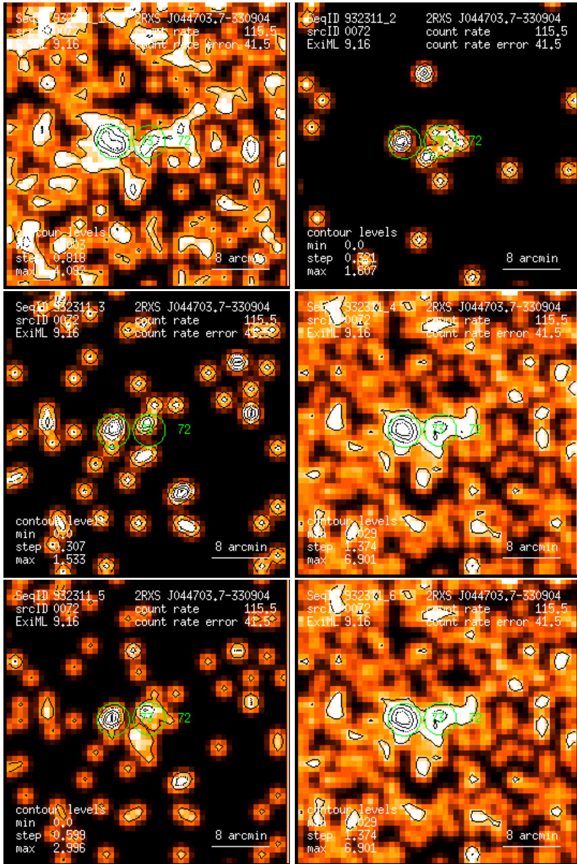
Figure 72: RASS 932311: detection 0072: band rate images, Gaussian filter: (1) PSPC channels 11 – 41, (2) 52 – 90, (3) 91 – 201, (4) 11 – 235, (5) 52 – 201, (6) 11 – 201. Broad band rates in counts/ks. Band rate contour levels in counts/ks/arcmin 2 .
