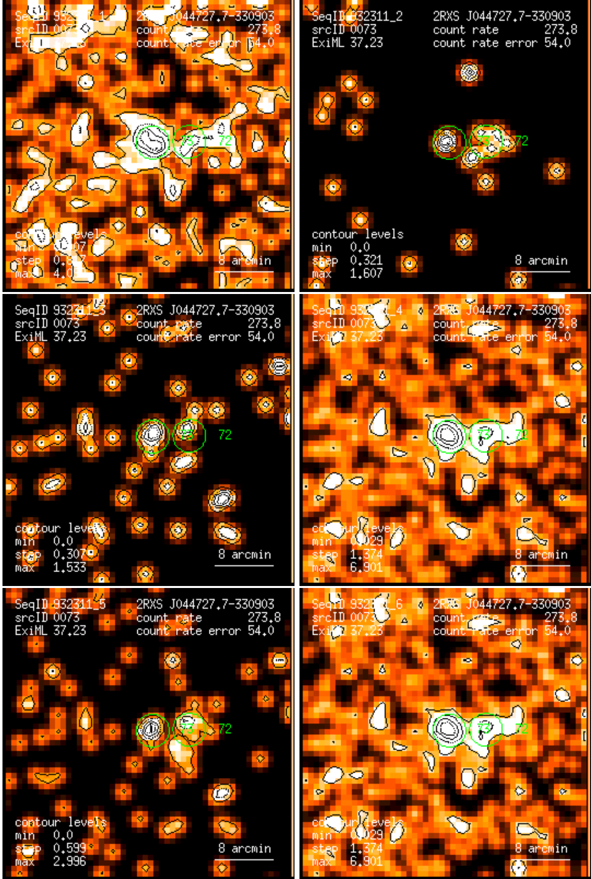
Figure 73: RASS 932311: detection 0073: band rate images, Gaussian filter: (1) PSPC channels 11 – 41, (2) 52 – 90, (3) 91 – 201, (4) 11 – 235, (5) 52 – 201, (6) 11 – 201. Broad band rates in counts/ks. Band rate contour levels in counts/ks/arcmin 2 .
