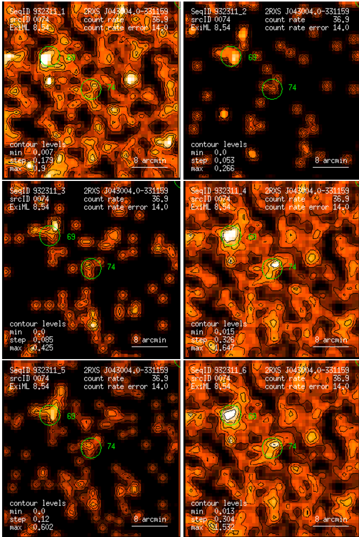
Figure 74: RASS 932311: detection 0074: band rate images, Gaussian filter: (1) PSPC channels 11 – 41, (2) 52 – 90, (3) 91 – 201, (4) 11 – 235, (5) 52 – 201, (6) 11 – 201. Broad band rates in counts/ks. Band rate contour levels in counts/ks/arcmin 2 .
