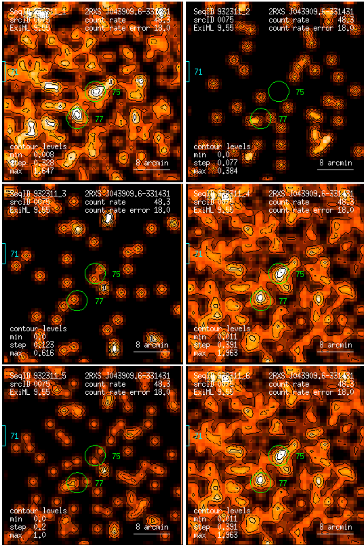
Figure 75: RASS 932311: detection 0075: band rate images, Gaussian filter: (1) PSPC channels 11 – 41, (2) 52 – 90, (3) 91 – 201, (4) 11 – 235, (5) 52 – 201, (6) 11 – 201. Broad band rates in counts/ks. Band rate contour levels in counts/ks/arcmin 2 .
