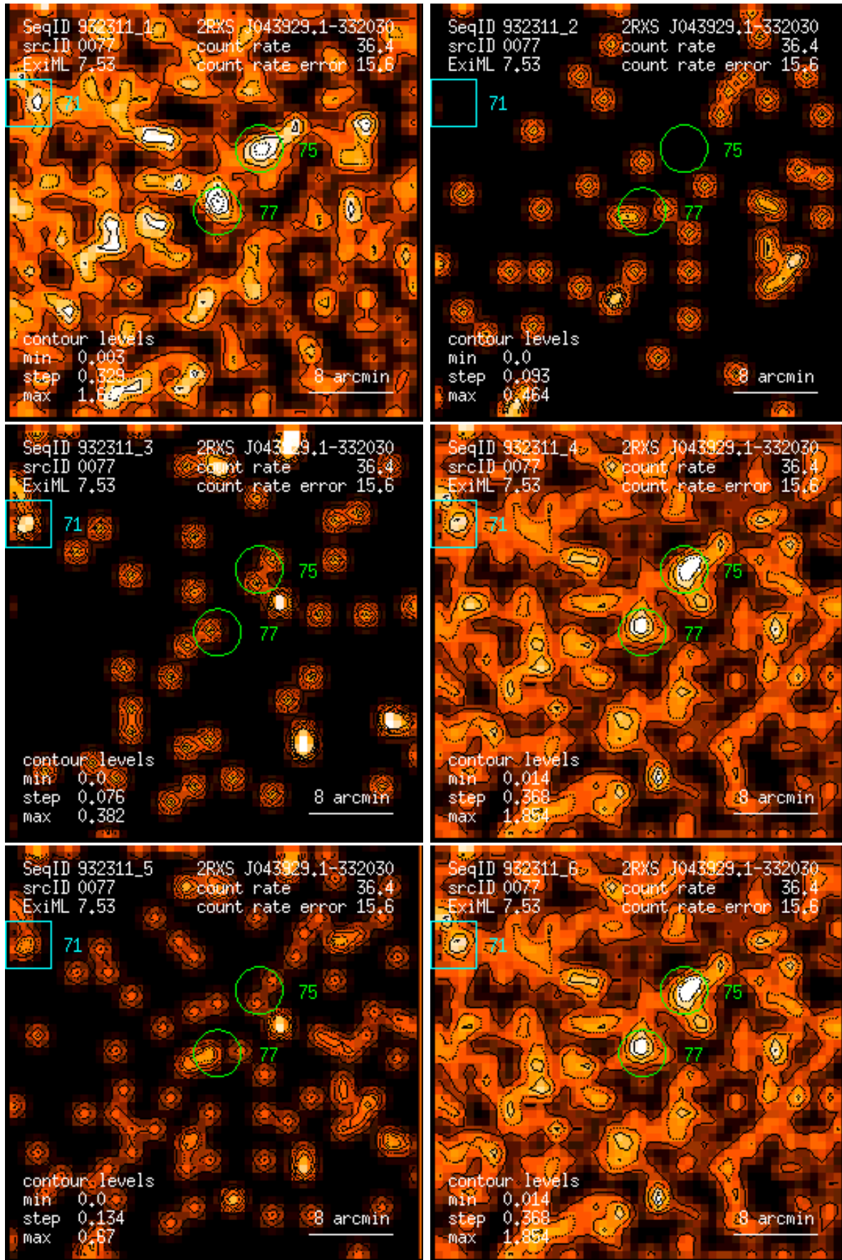
Figure 77: RASS 932311: detection 0077: band rate images, Gaussian filter: (1) PSPC channels 11 – 41, (2) 52 – 90, (3) 91 – 201, (4) 11 – 235, (5) 52 – 201, (6) 11 – 201. Broad band rates in counts/ks. Band rate contour levels in counts/ks/arcmin 2 .
