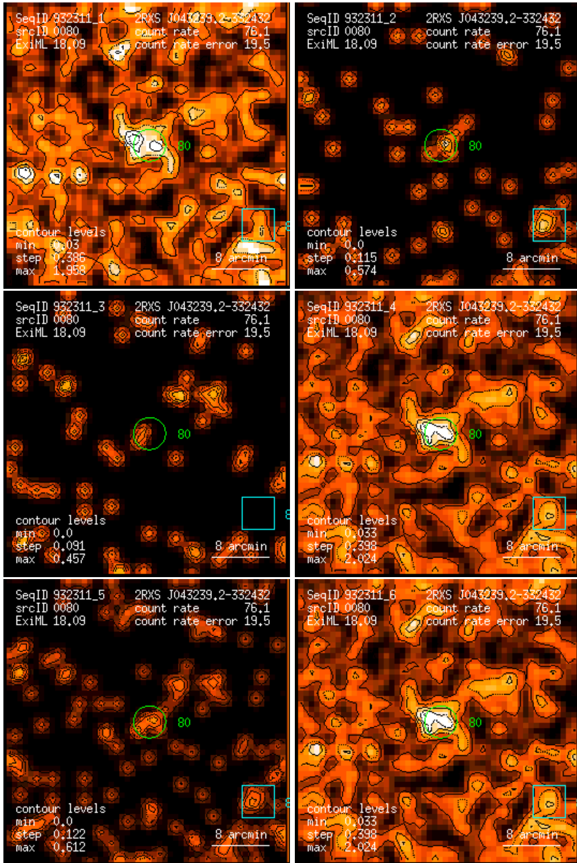
Figure 80: RASS 932311: detection 0080: band rate images, Gaussian filter: (1) PSPC channels 11 – 41, (2) 52 – 90, (3) 91 – 201, (4) 11 – 235, (5) 52 – 201, (6) 11 – 201. Broad band rates in counts/ks. Band rate contour levels in counts/ks/arcmin 2 .
