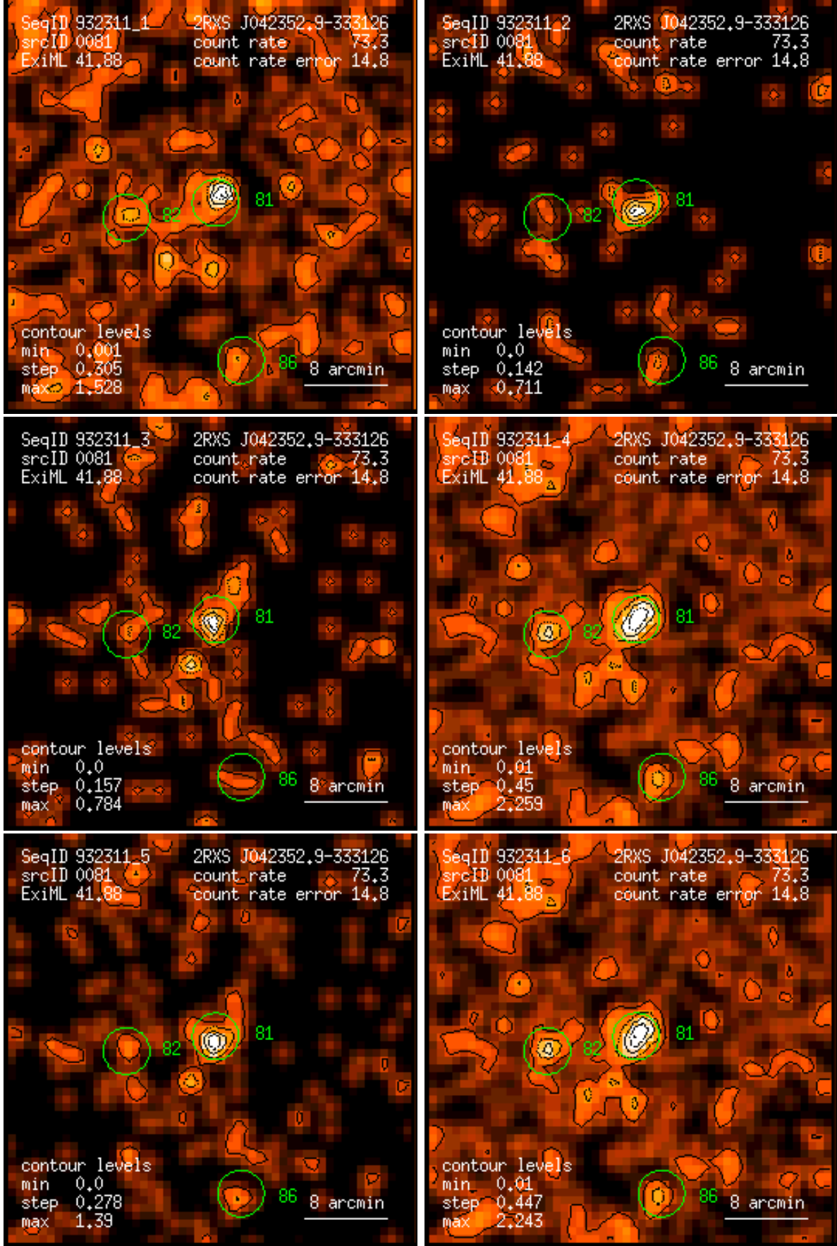
Figure 81: RASS 932311: detection 0081: band rate images, Gaussian filter: (1) PSPC channels 11 – 41, (2) 52 – 90, (3) 91 – 201, (4) 11 – 235, (5) 52 – 201, (6) 11 – 201. Broad band rates in counts/ks. Band rate contour levels in counts/ks/arcmin 2 .
