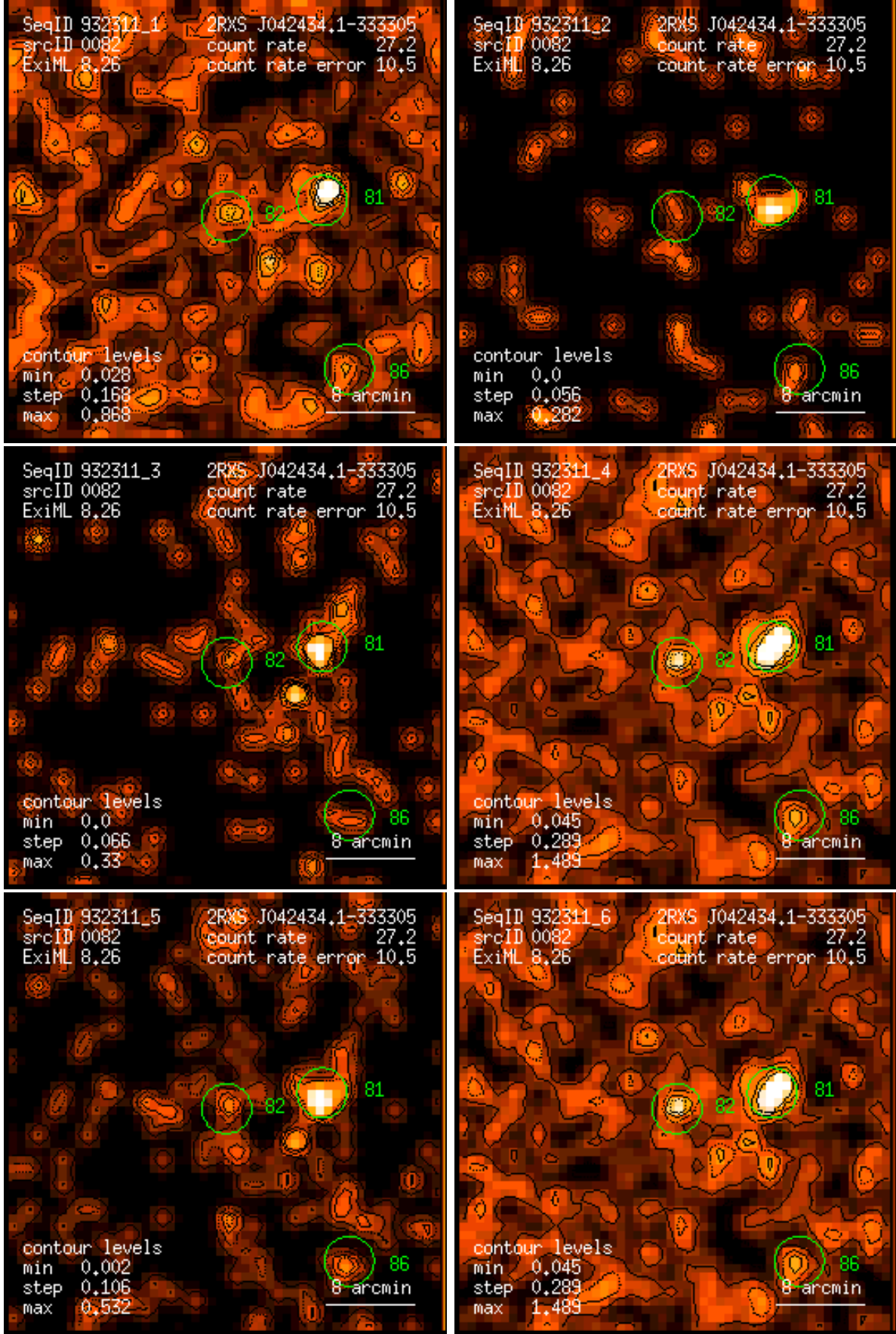
Figure 82: RASS 932311: detection 0082: band rate images, Gaussian filter: (1) PSPC channels 11 – 41, (2) 52 – 90, (3) 91 – 201, (4) 11 – 235, (5) 52 – 201, (6) 11 – 201. Broad band rates in counts/ks. Band rate contour levels in counts/ks/arcmin 2 .
