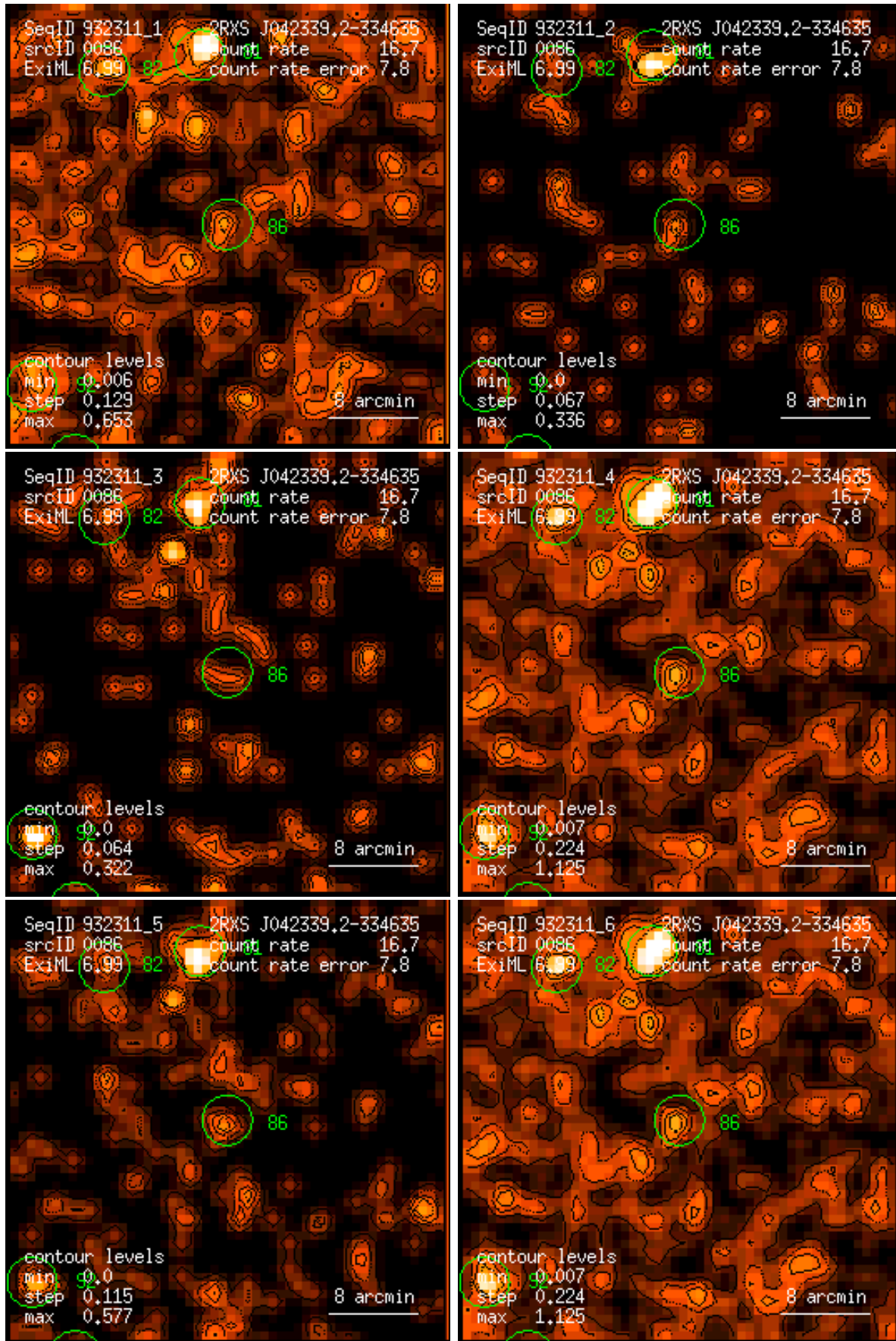
Figure 86: RASS 932311: detection 0086: band rate images, Gaussian filter: (1) PSPC channels 11 – 41, (2) 52 – 90, (3) 91 – 201, (4) 11 – 235, (5) 52 – 201, (6) 11 – 201. Broad band rates in counts/ks. Band rate contour levels in counts/ks/arcmin 2 .
