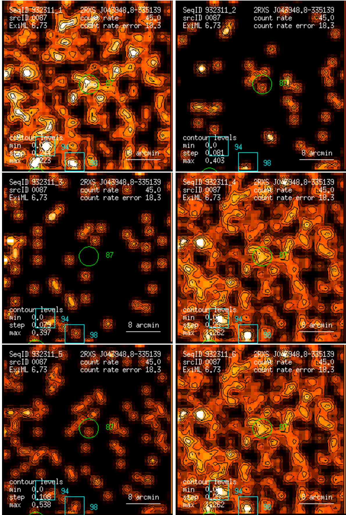
Figure 87: RASS 932311: detection 0087: band rate images, Gaussian filter: (1) PSPC channels 11 – 41, (2) 52 – 90, (3) 91 – 201, (4) 11 – 235, (5) 52 – 201, (6) 11 – 201. Broad band rates in counts/ks. Band rate contour levels in counts/ks/arcmin 2 .
