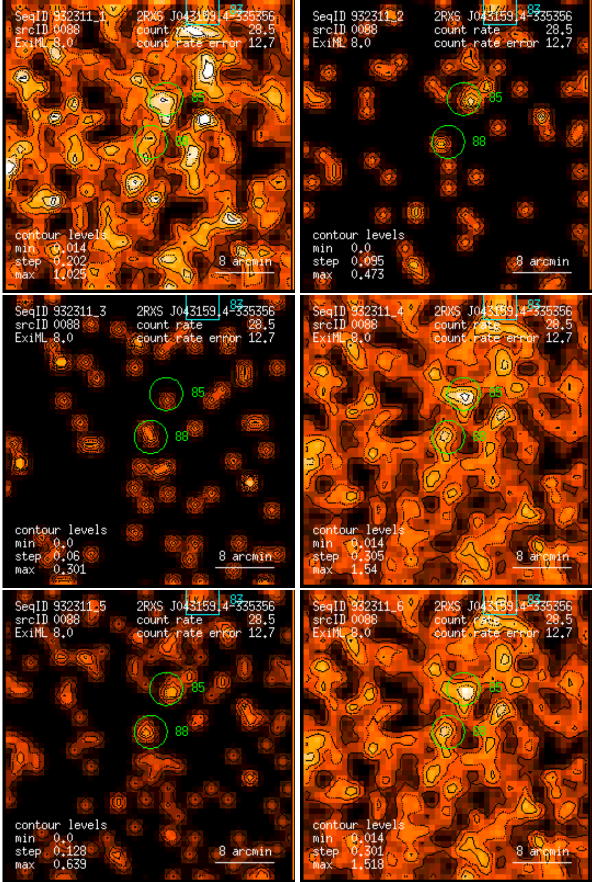
Figure 88: RASS 932311: detection 0088: band rate images, Gaussian filter: (1) PSPC channels 11 – 41, (2) 52 – 90, (3) 91 – 201, (4) 11 – 235, (5) 52 – 201, (6) 11 – 201. Broad band rates in counts/ks. Band rate contour levels in counts/ks/arcmin 2 .
