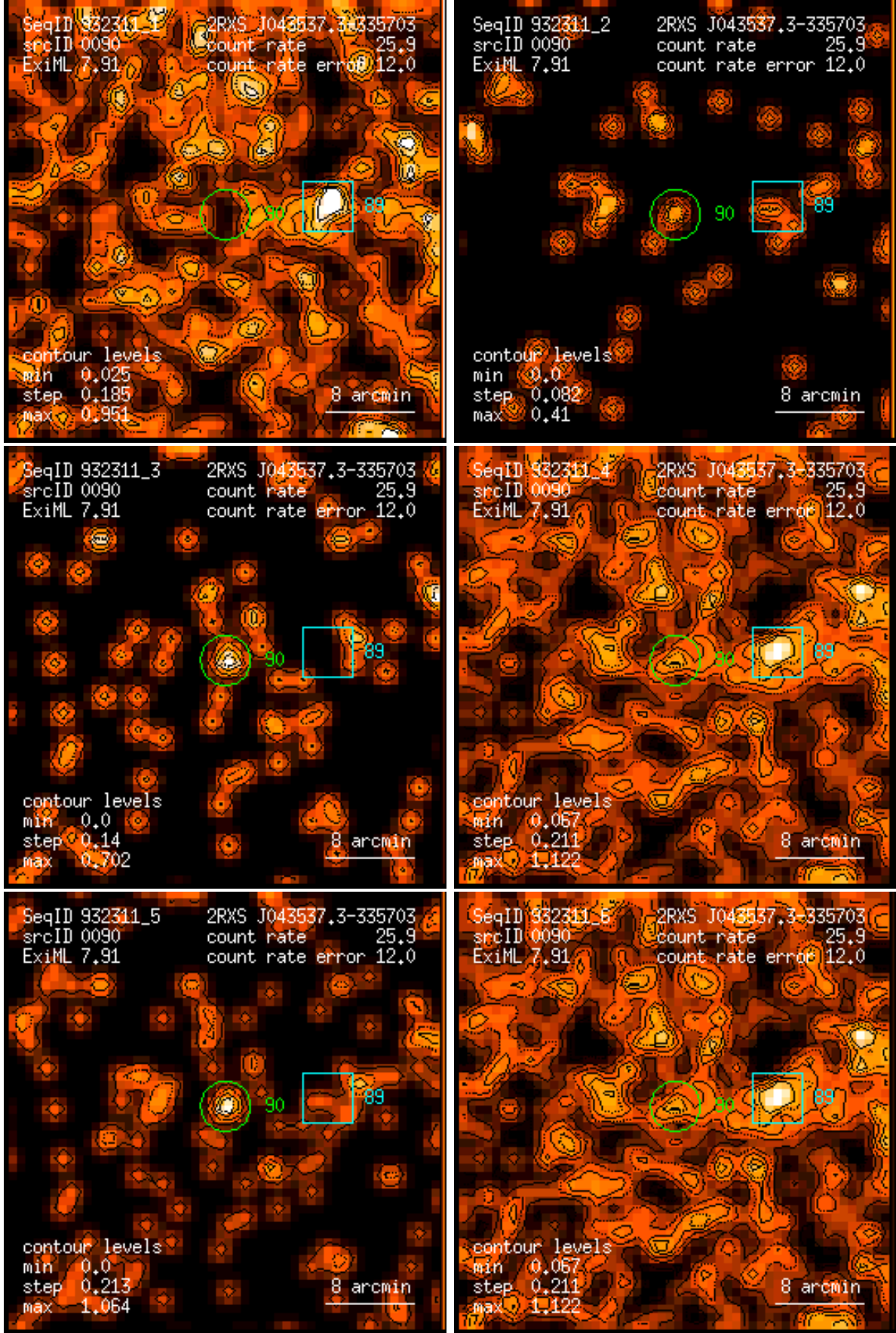
Figure 90: RASS 932311: detection 0090: band rate images, Gaussian filter: (1) PSPC channels 11 – 41, (2) 52 – 90, (3) 91 – 201, (4) 11 – 235, (5) 52 – 201, (6) 11 – 201. Broad band rates in counts/ks. Band rate contour levels in counts/ks/arcmin 2 .
