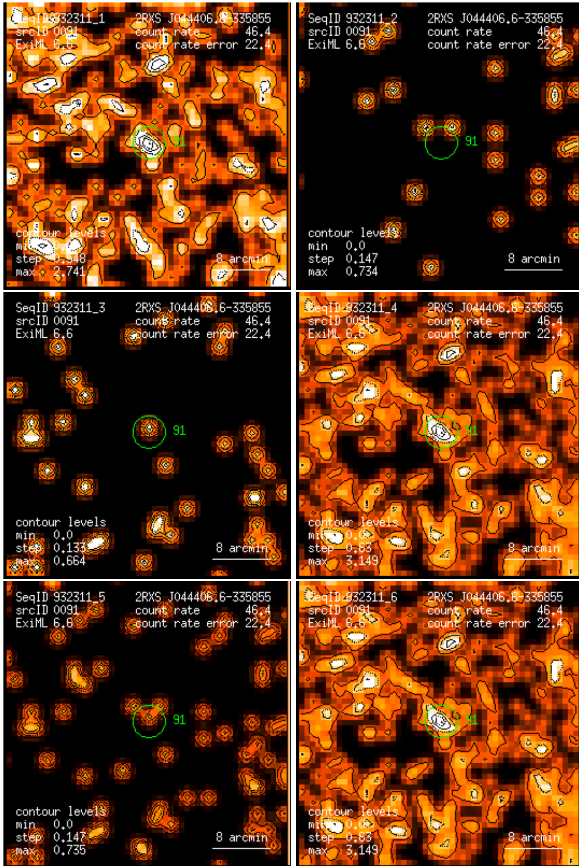
Figure 91: RASS 932311: detection 0091: band rate images, Gaussian filter: (1) PSPC channels 11 – 41, (2) 52 – 90, (3) 91 – 201, (4) 11 – 235, (5) 52 – 201, (6) 11 – 201. Broad band rates in counts/ks. Band rate contour levels in counts/ks/arcmin 2 .
