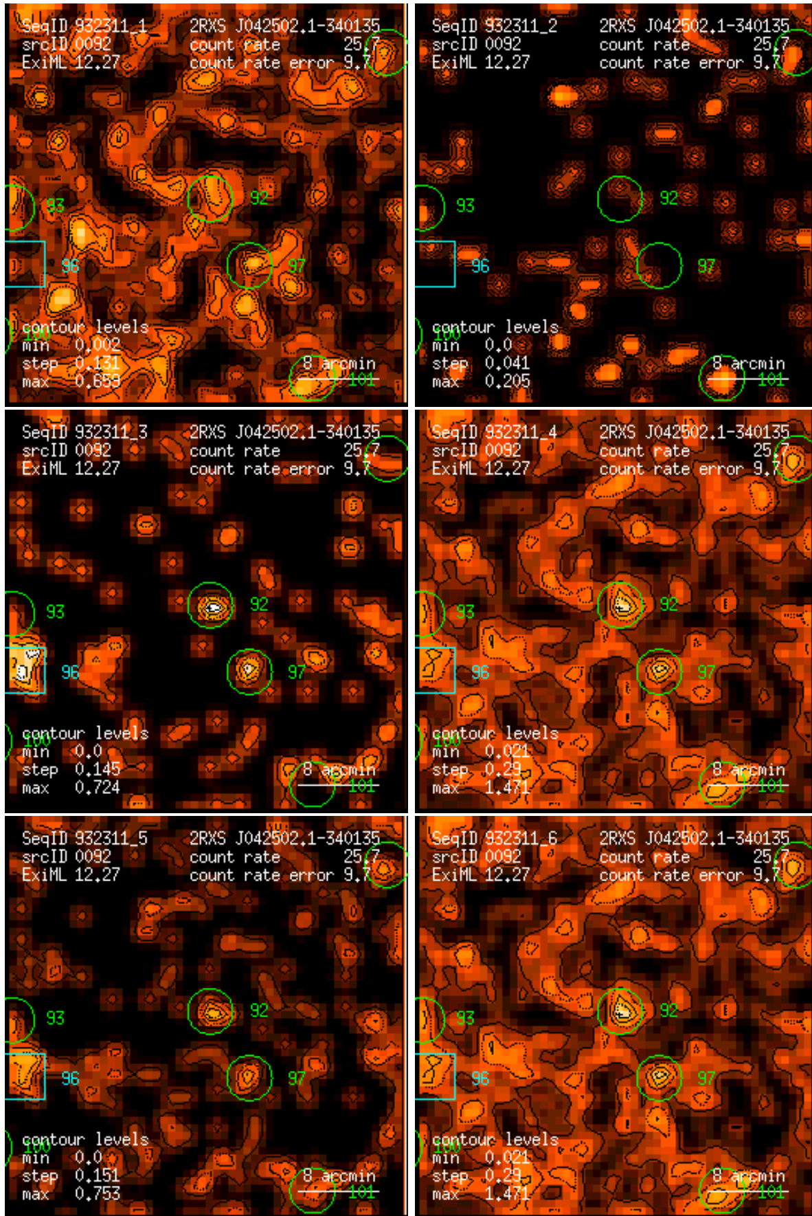
Figure 92: RASS 932311: detection 0092: band rate images, Gaussian filter: (1) PSPC channels 11 – 41, (2) 52 – 90, (3) 91 – 201, (4) 11 – 235, (5) 52 – 201, (6) 11 – 201. Broad band rates in counts/ks. Band rate contour levels in counts/ks/arcmin 2 .
