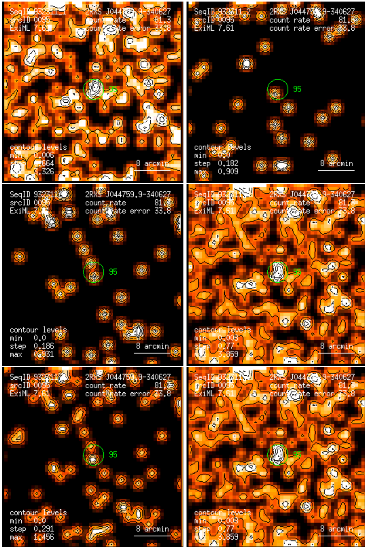
Figure 95: RASS 932311: detection 0095: band rate images, Gaussian filter: (1) PSPC channels 11 – 41, (2) 52 – 90, (3) 91 – 201, (4) 11 – 235, (5) 52 – 201, (6) 11 – 201. Broad band rates in counts/ks. Band rate contour levels in counts/ks/arcmin 2 .
