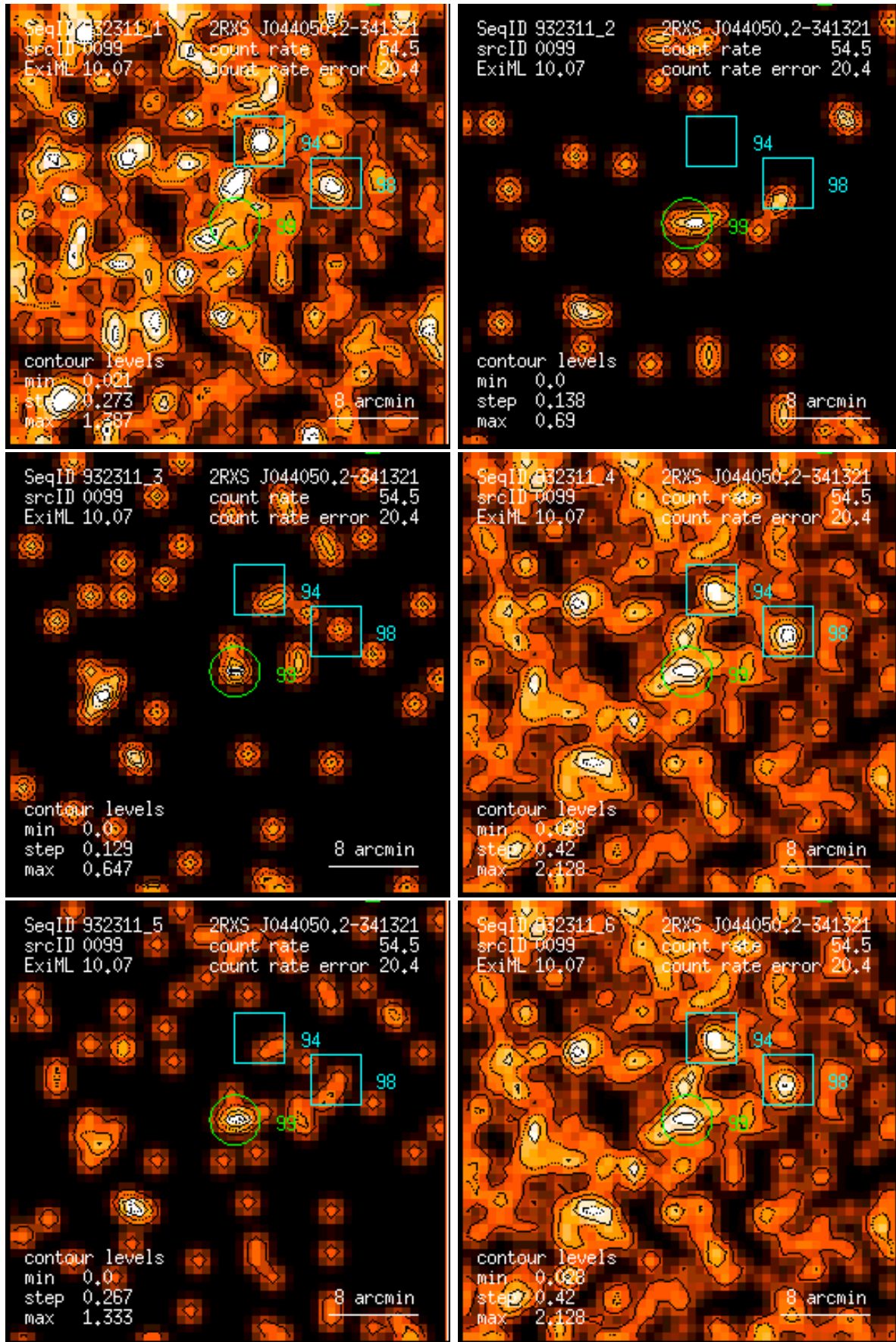
Figure 99: RASS 932311: detection 0099: band rate images, Gaussian filter: (1) PSPC channels 11 – 41, (2) 52 – 90, (3) 91 – 201, (4) 11 – 235, (5) 52 – 201, (6) 11 – 201. Broad band rates in counts/ks. Band rate contour levels in counts/ks/arcmin 2 .
